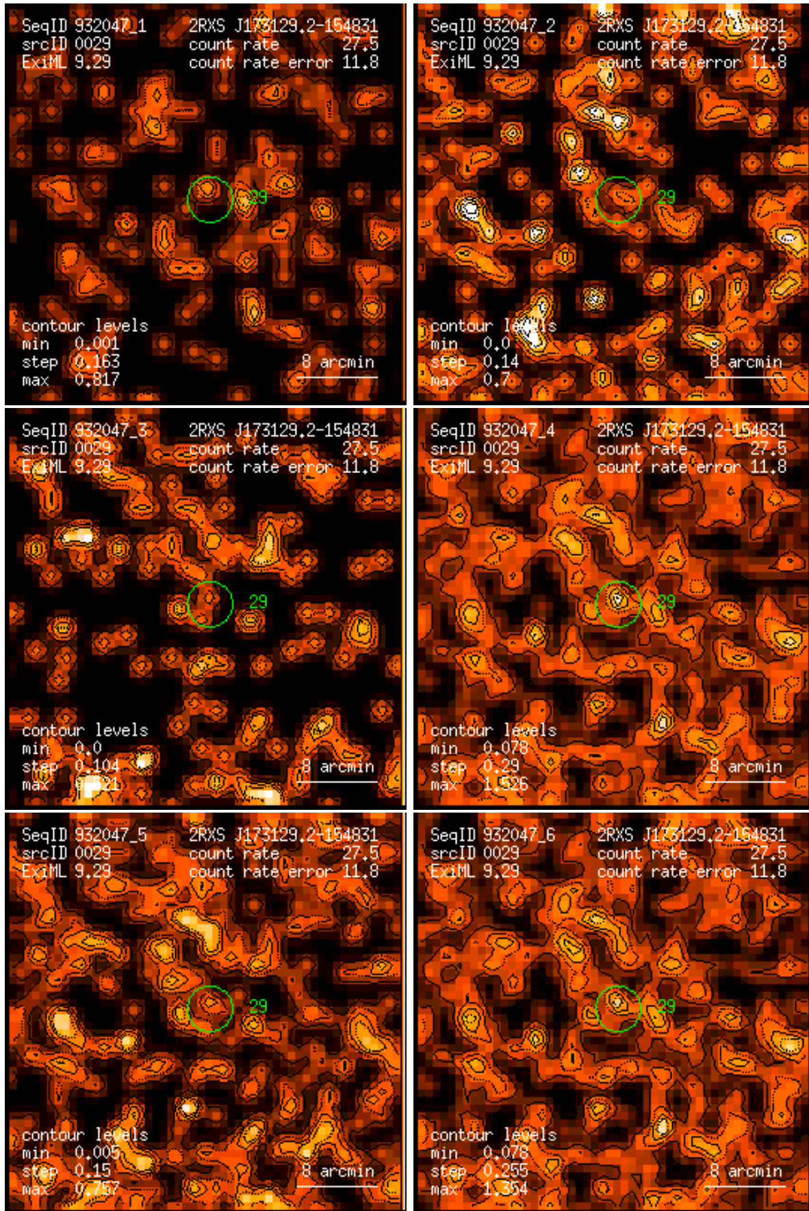
Figure 29: RASS 932047: detection 0029: band rate images, Gaussian filter: (1) PSPC channels 11 – 41, (2) 52 – 90, (3) 91 – 201, (4) 11 – 235, (5) 52 – 201, (6) 11 – 201. Broad band rates in counts/ks. Band rate contour levels in counts/ks/arcmin 2 .
