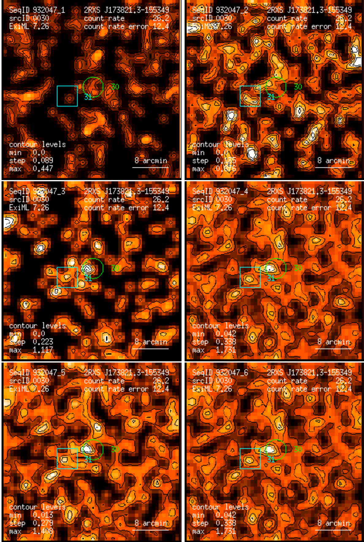
Figure 30: RASS 932047: detection 0030: band rate images, Gaussian filter: (1) PSPC channels 11 – 41, (2) 52 – 90, (3) 91 – 201, (4) 11 – 235, (5) 52 – 201, (6) 11 – 201. Broad band rates in counts/ks. Band rate contour levels in counts/ks/arcmin 2 .
