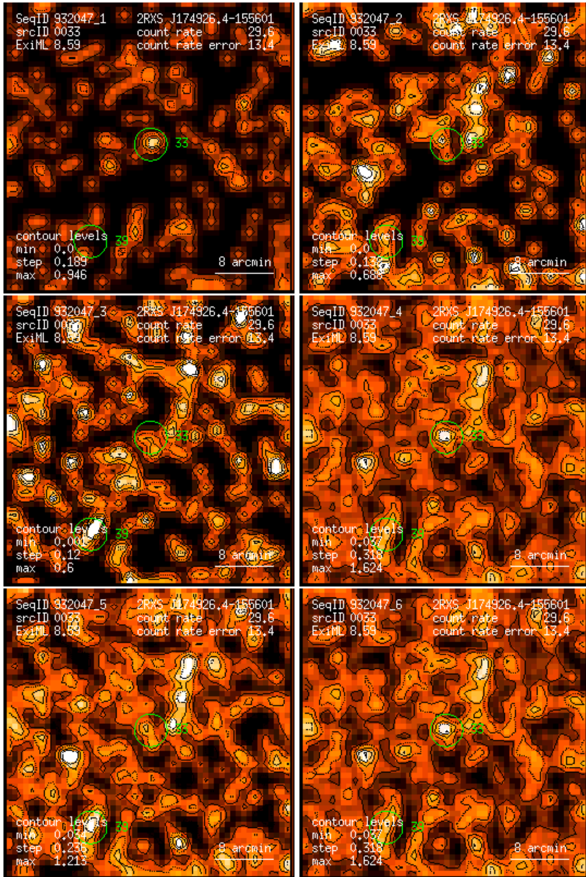
Figure 33: RASS 932047: detection 0033: band rate images, Gaussian filter: (1) PSPC channels 11 – 41, (2) 52 – 90, (3) 91 – 201, (4) 11 – 235, (5) 52 – 201, (6) 11 – 201. Broad band rates in counts/ks. Band rate contour levels in counts/ks/arcmin 2 .
