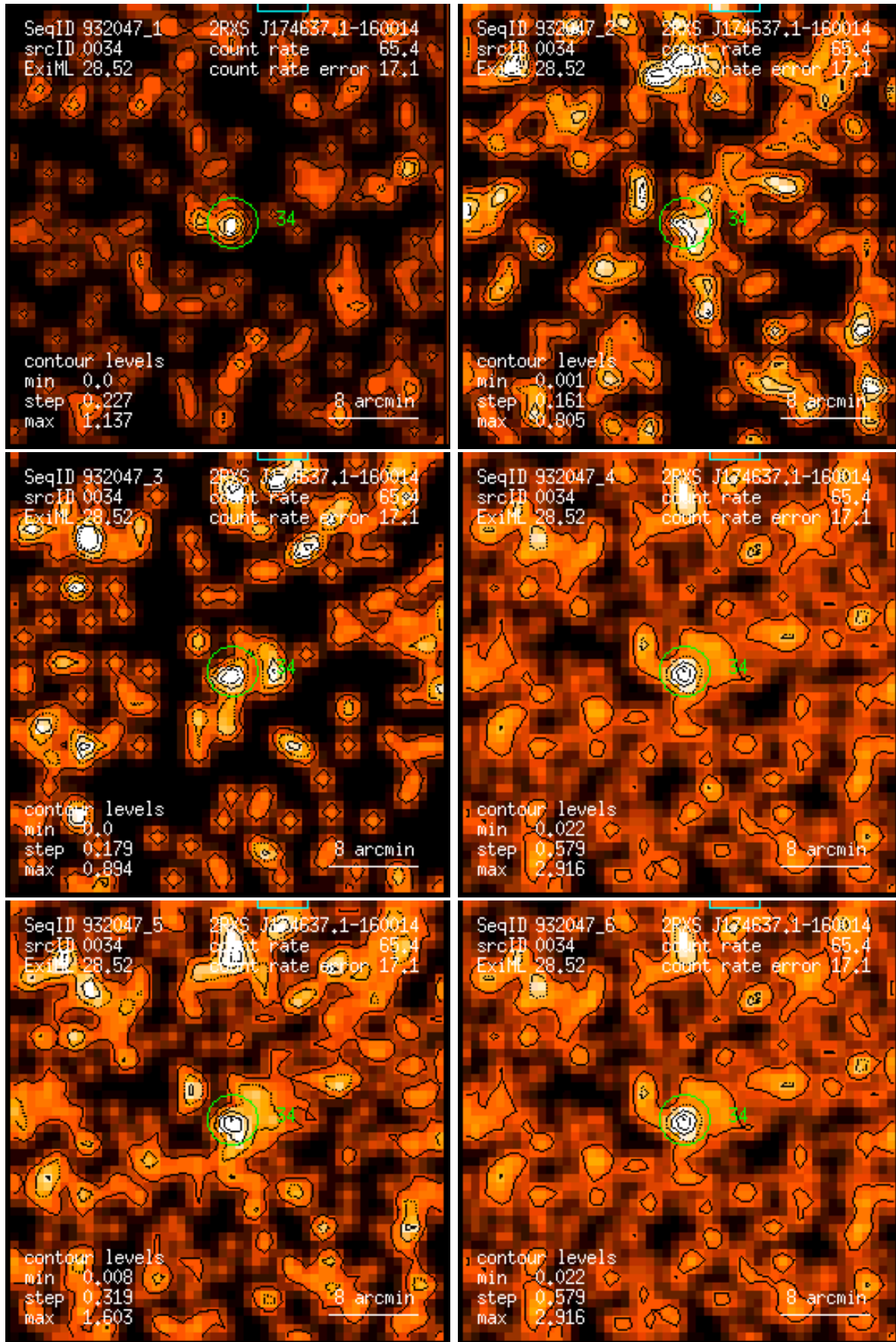
Figure 34: RASS 932047: detection 0034: band rate images, Gaussian filter: (1) PSPC channels 11 – 41, (2) 52 – 90, (3) 91 – 201, (4) 11 – 235, (5) 52 – 201, (6) 11 – 201. Broad band rates in counts/ks. Band rate contour levels in counts/ks/arcmin 2 .
