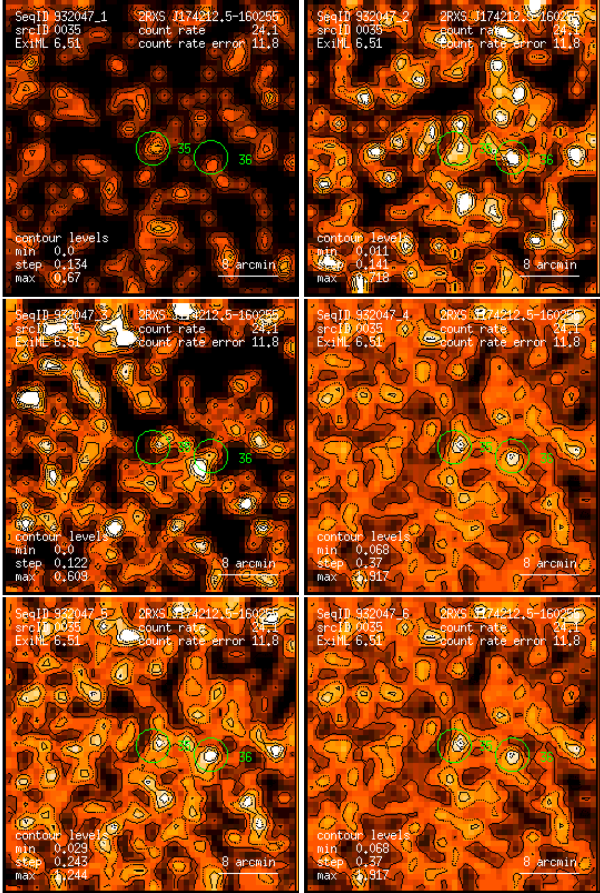
Figure 35: RASS 932047: detection 0035: band rate images, Gaussian filter: (1) PSPC channels 11 – 41, (2) 52 – 90, (3) 91 – 201, (4) 11 – 235, (5) 52 – 201, (6) 11 – 201. Broad band rates in counts/ks. Band rate contour levels in counts/ks/arcmin 2 .
