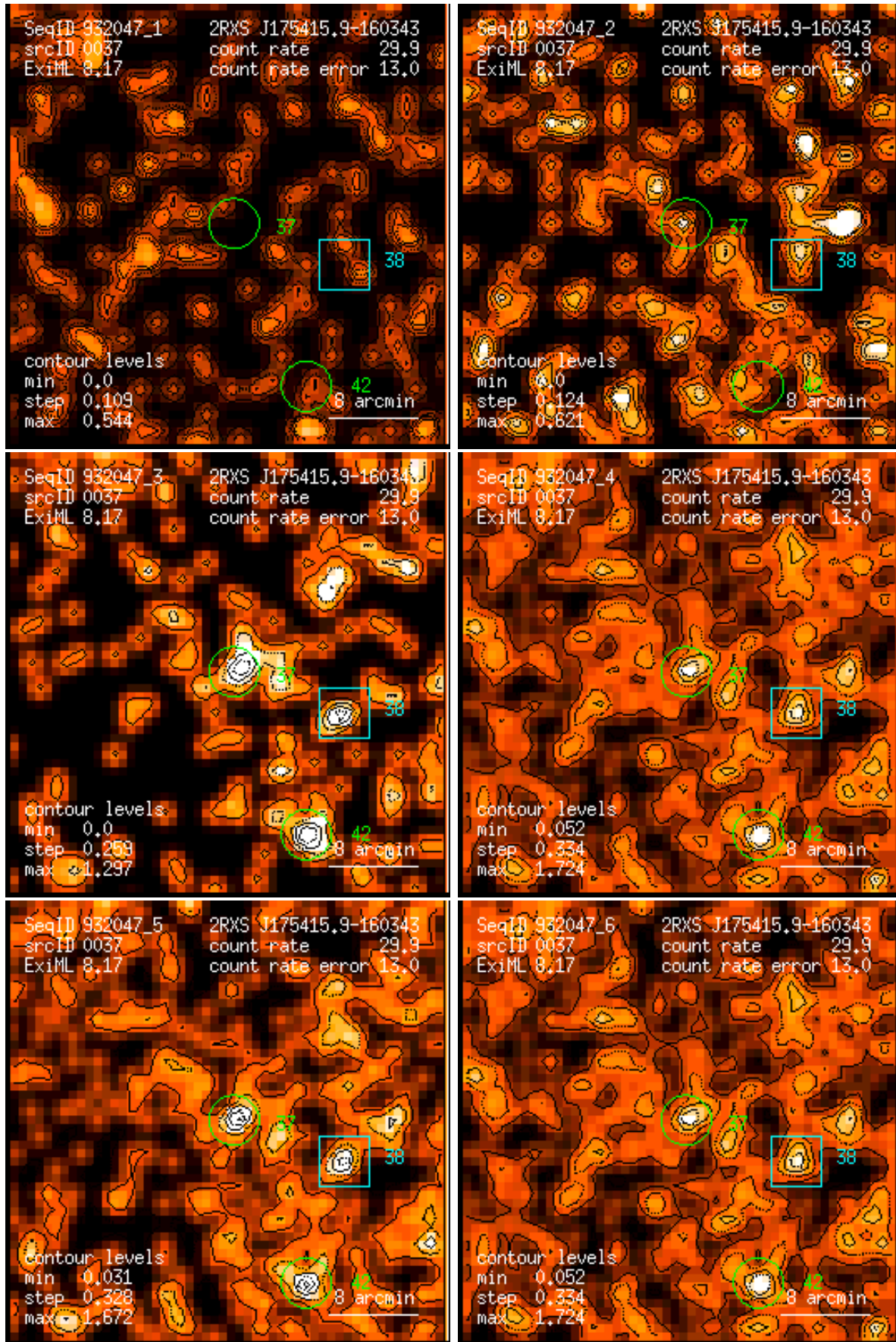
Figure 37: RASS 932047: detection 0037: band rate images, Gaussian filter: (1) PSPC channels 11 – 41, (2) 52 – 90, (3) 91 – 201, (4) 11 – 235, (5) 52 – 201, (6) 11 – 201. Broad band rates in counts/ks. Band rate contour levels in counts/ks/arcmin 2 .
