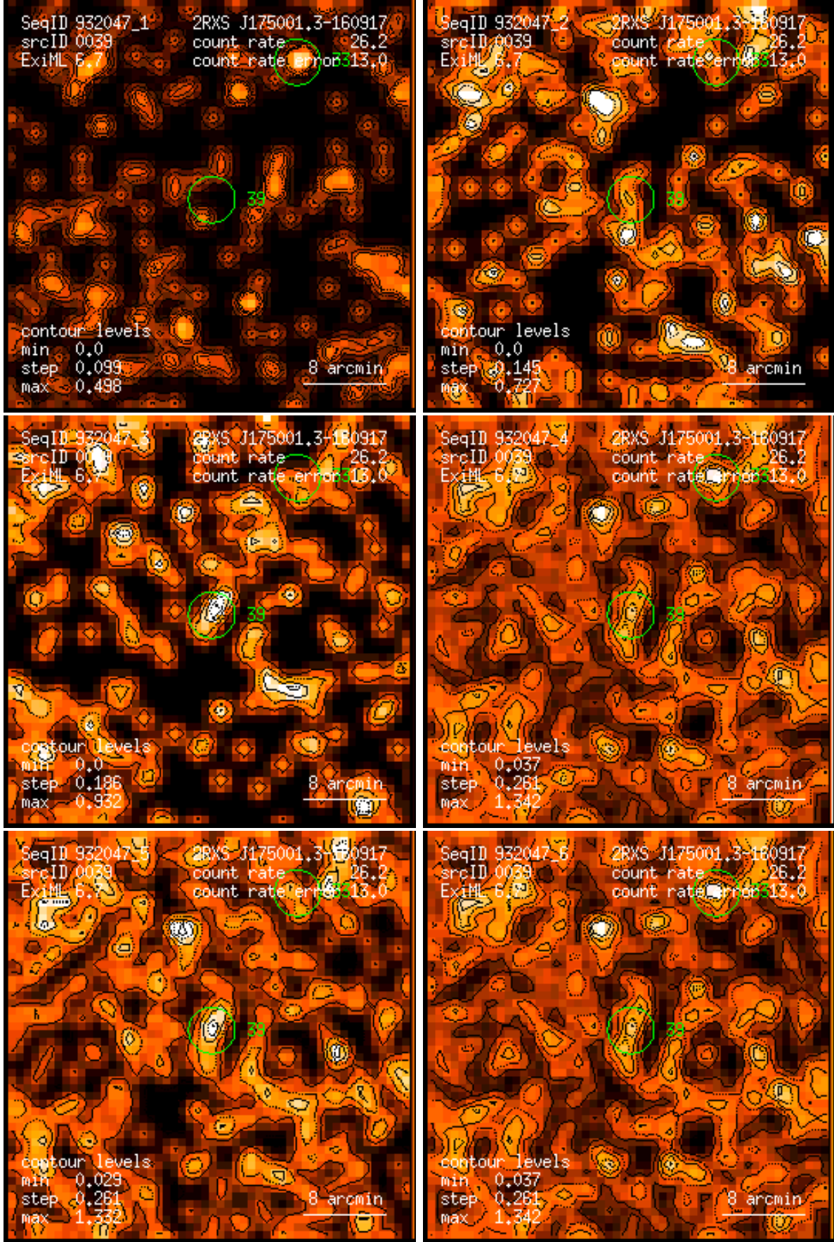
Figure 39: RASS 932047: detection 0039: band rate images, Gaussian filter: (1) PSPC channels 11 – 41, (2) 52 – 90, (3) 91 – 201, (4) 11 – 235, (5) 52 – 201, (6) 11 – 201. Broad band rates in counts/ks. Band rate contour levels in counts/ks/arcmin 2 .
