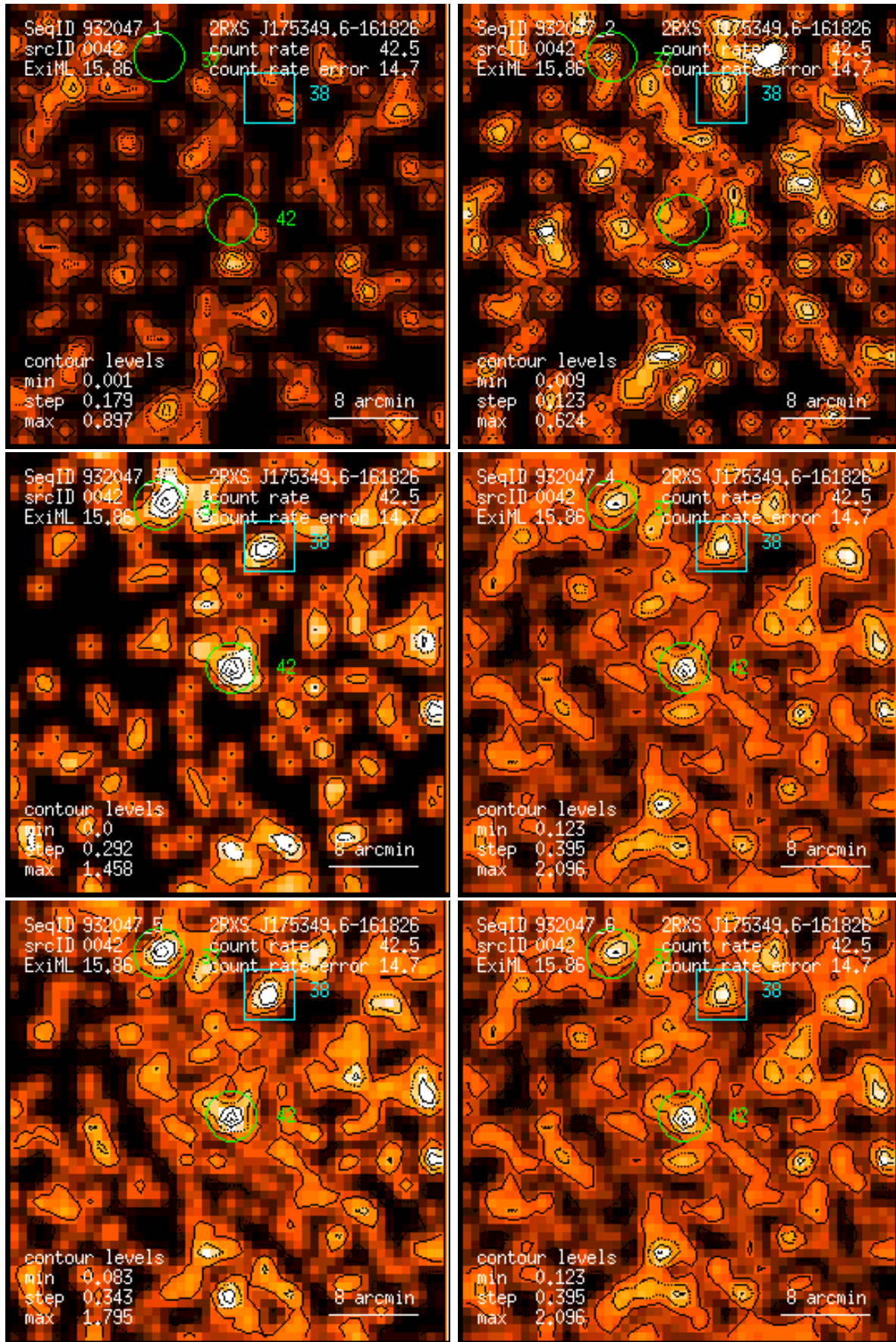
Figure 42: RASS 932047: detection 0042: band rate images, Gaussian filter: (1) PSPC channels 11 – 41, (2) 52 – 90, (3) 91 – 201, (4) 11 – 235, (5) 52 – 201, (6) 11 – 201. Broad band rates in counts/ks. Band rate contour levels in counts/ks/arcmin 2 .
