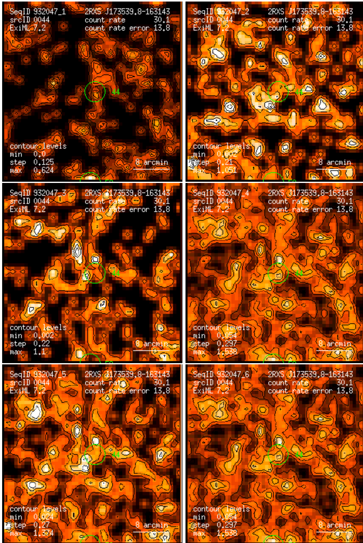
Figure 44: RASS 932047: detection 0044: band rate images, Gaussian filter: (1) PSPC channels 11 – 41, (2) 52 – 90, (3) 91 – 201, (4) 11 – 235, (5) 52 – 201, (6) 11 – 201. Broad band rates in counts/ks. Band rate contour levels in counts/ks/arcmin 2 .
