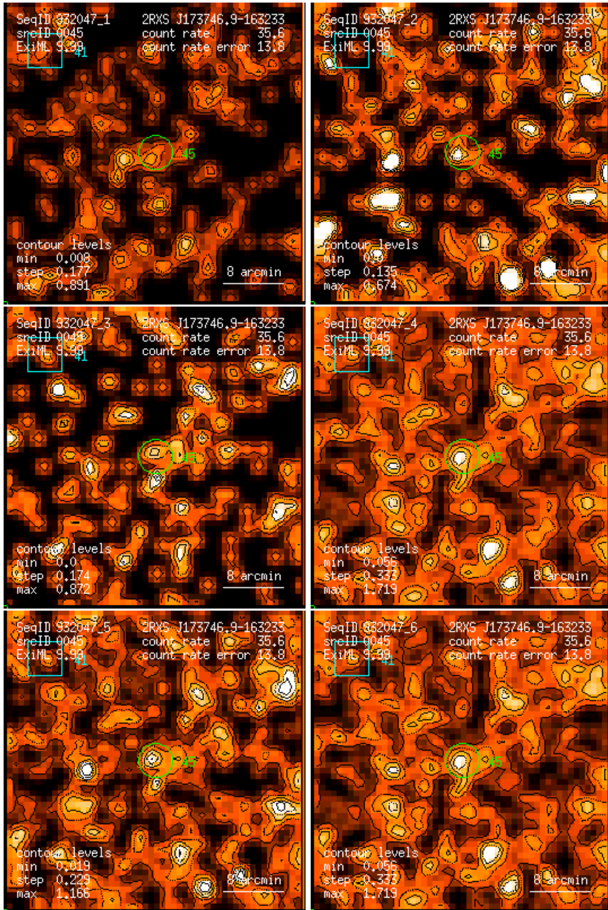
Figure 45: RASS 932047: detection 0045: band rate images, Gaussian filter: (1) PSPC channels 11 – 41, (2) 52 – 90, (3) 91 – 201, (4) 11 – 235, (5) 52 – 201, (6) 11 – 201. Broad band rates in counts/ks. Band rate contour levels in counts/ks/arcmin 2 .
