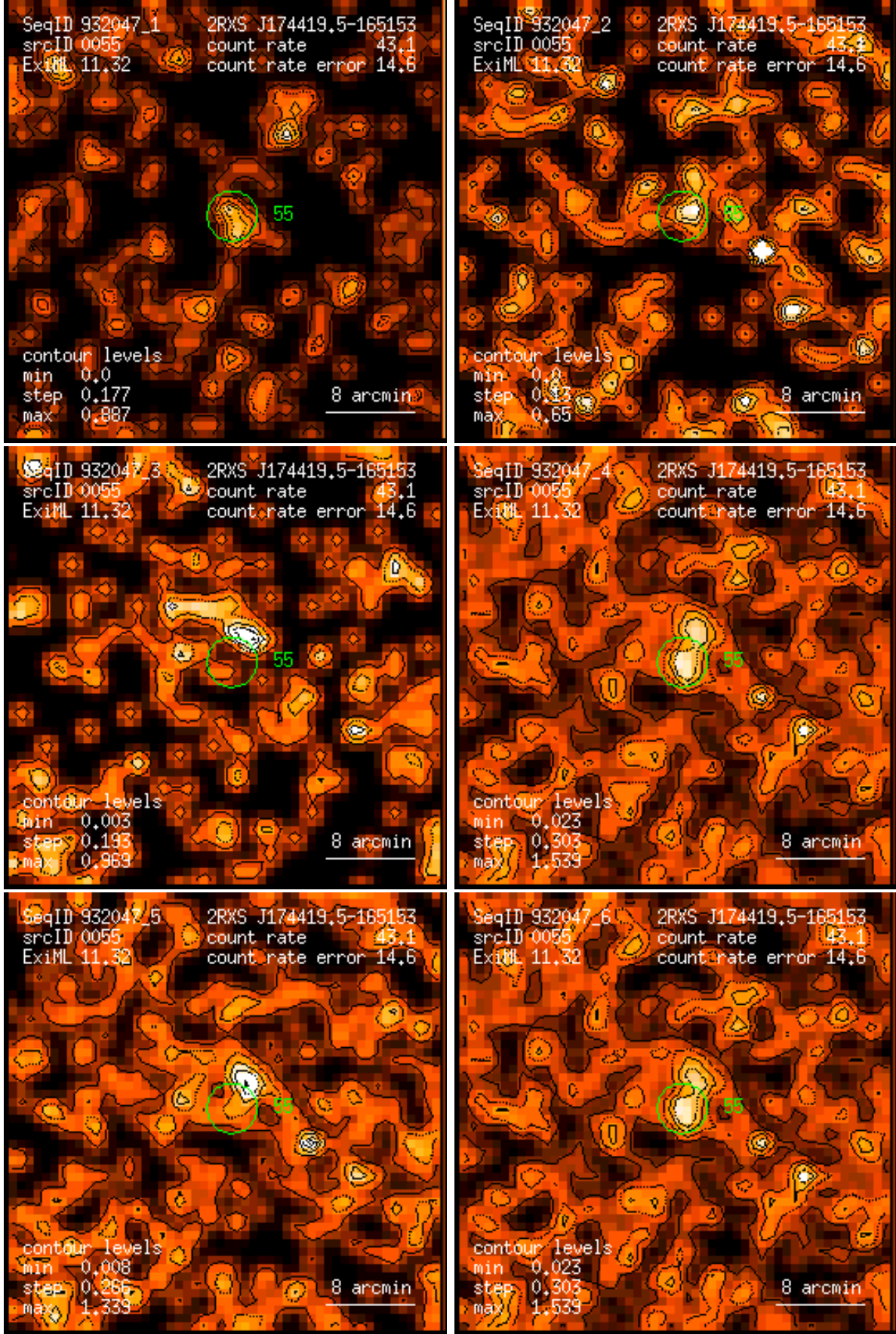
Figure 55: RASS 932047: detection 0055: band rate images, Gaussian filter: (1) PSPC channels 11 – 41, (2) 52 – 90, (3) 91 – 201, (4) 11 – 235, (5) 52 – 201, (6) 11 – 201. Broad band rates in counts/ks. Band rate contour levels in counts/ks/arcmin 2 .
