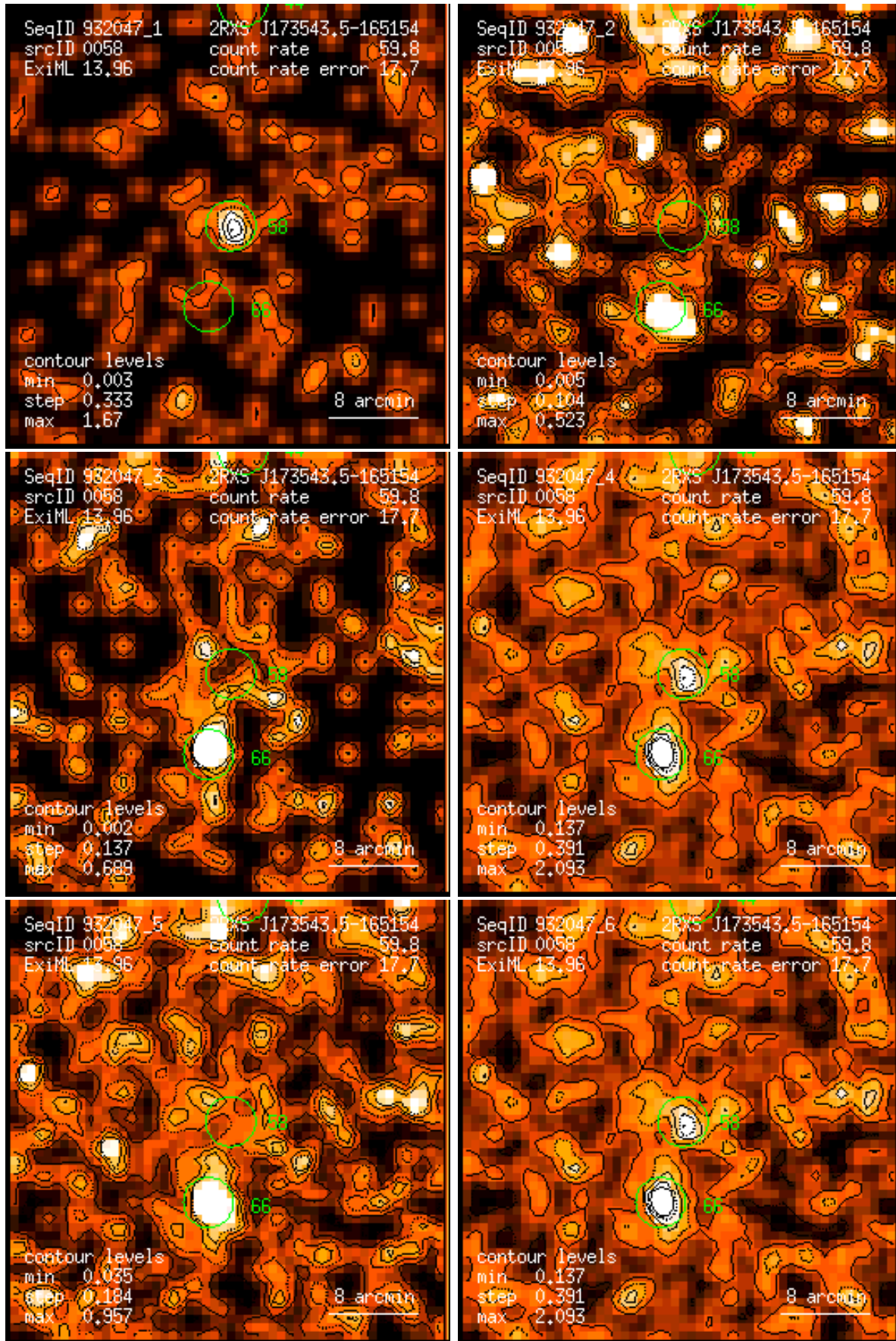
Figure 58: RASS 932047: detection 0058: band rate images, Gaussian filter: (1) PSPC channels 11 – 41, (2) 52 – 90, (3) 91 – 201, (4) 11 – 235, (5) 52 – 201, (6) 11 – 201. Broad band rates in counts/ks. Band rate contour levels in counts/ks/arcmin 2 .
