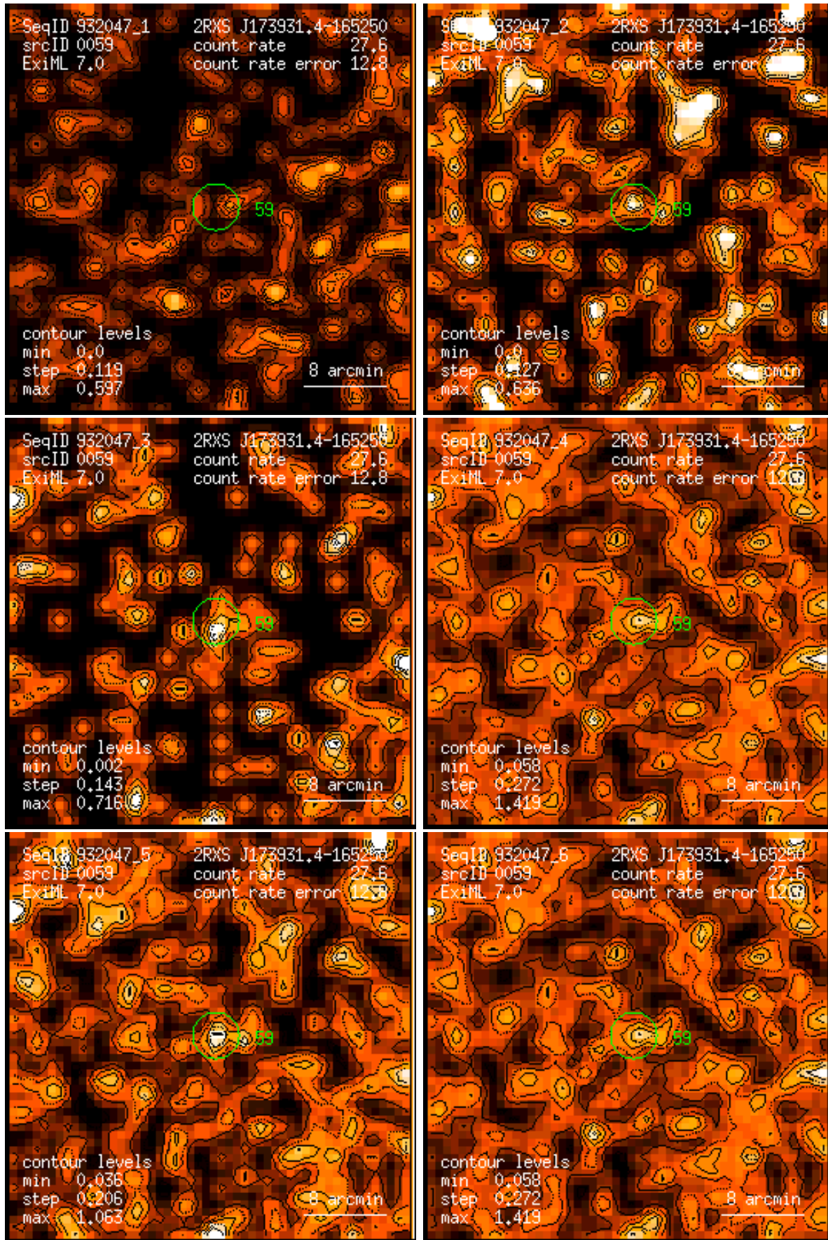
Figure 59: RASS 932047: detection 0059: band rate images, Gaussian filter: (1) PSPC channels 11 – 41, (2) 52 – 90, (3) 91 – 201, (4) 11 – 235, (5) 52 – 201, (6) 11 – 201. Broad band rates in counts/ks. Band rate contour levels in counts/ks/arcmin 2 .
