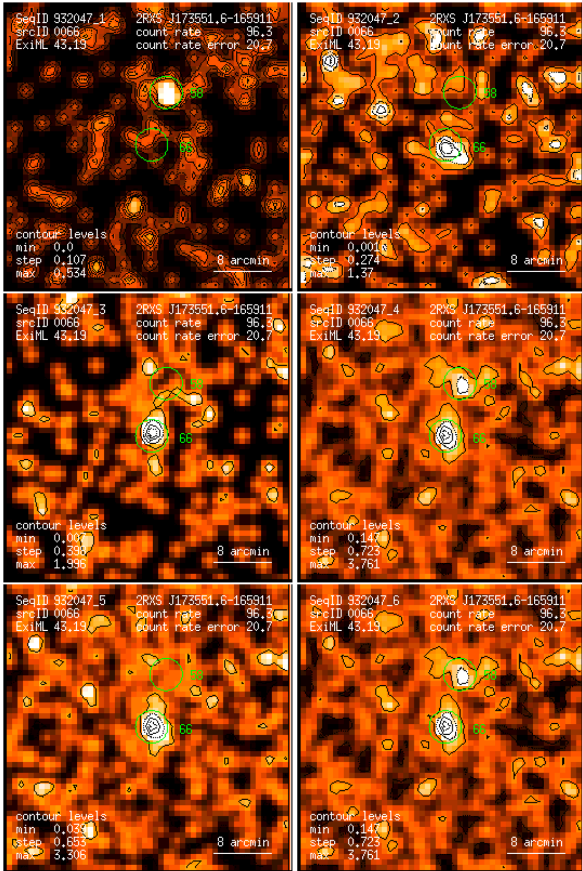
Figure 66: RASS 932047: detection 0066: band rate images, Gaussian filter: (1) PSPC channels 11 – 41, (2) 52 – 90, (3) 91 – 201, (4) 11 – 235, (5) 52 – 201, (6) 11 – 201. Broad band rates in counts/ks. Band rate contour levels in counts/ks/arcmin 2 .
