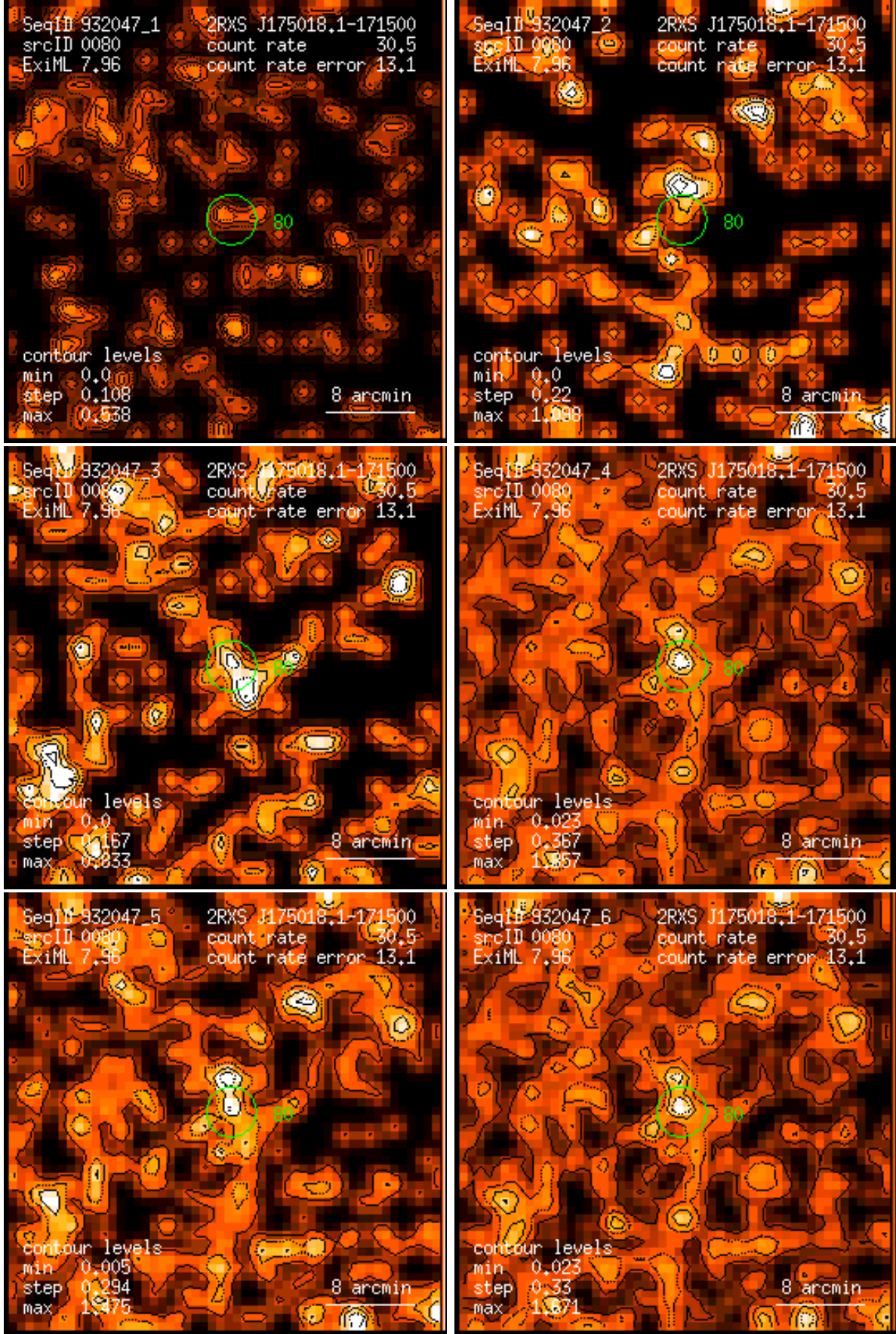
Figure 80: RASS 932047: detection 0080: band rate images, Gaussian filter: (1) PSPC channels 11 – 41, (2) 52 – 90, (3) 91 – 201, (4) 11 – 235, (5) 52 – 201, (6) 11 – 201. Broad band rates in counts/ks. Band rate contour levels in counts/ks/arcmin 2 .
