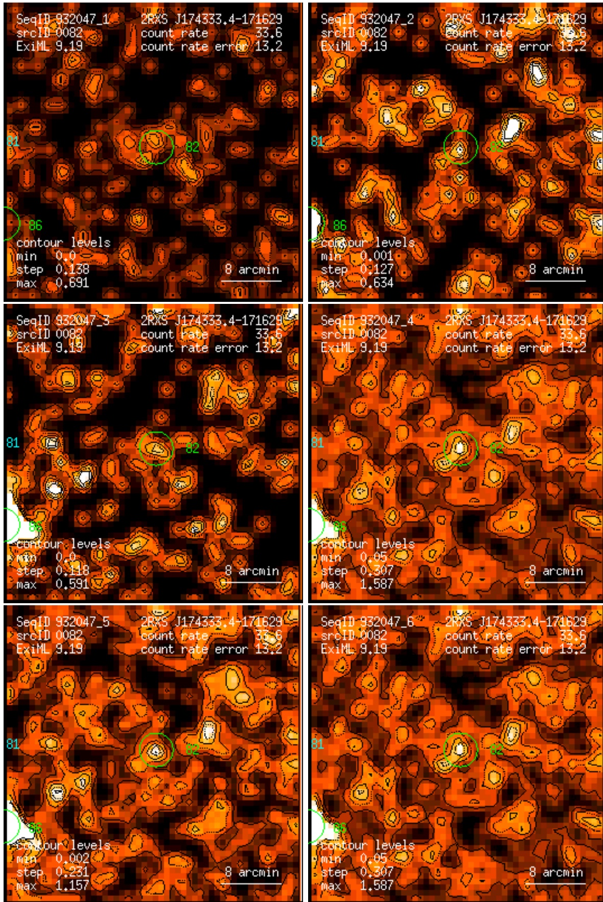
Figure 82: RASS 932047: detection 0082: band rate images, Gaussian filter: (1) PSPC channels 11 – 41, (2) 52 – 90, (3) 91 – 201, (4) 11 – 235, (5) 52 – 201, (6) 11 – 201. Broad band rates in counts/ks. Band rate contour levels in counts/ks/arcmin 2 .
