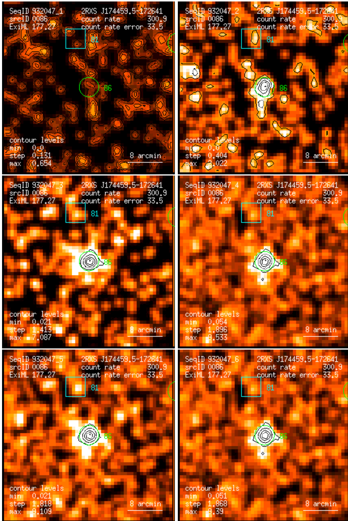
Figure 86: RASS 932047: detection 0086: band rate images, Gaussian filter: (1) PSPC channels 11 – 41, (2) 52 – 90, (3) 91 – 201, (4) 11 – 235, (5) 52 – 201, (6) 11 – 201. Broad band rates in counts/ks. Band rate contour levels in counts/ks/arcmin 2 .
