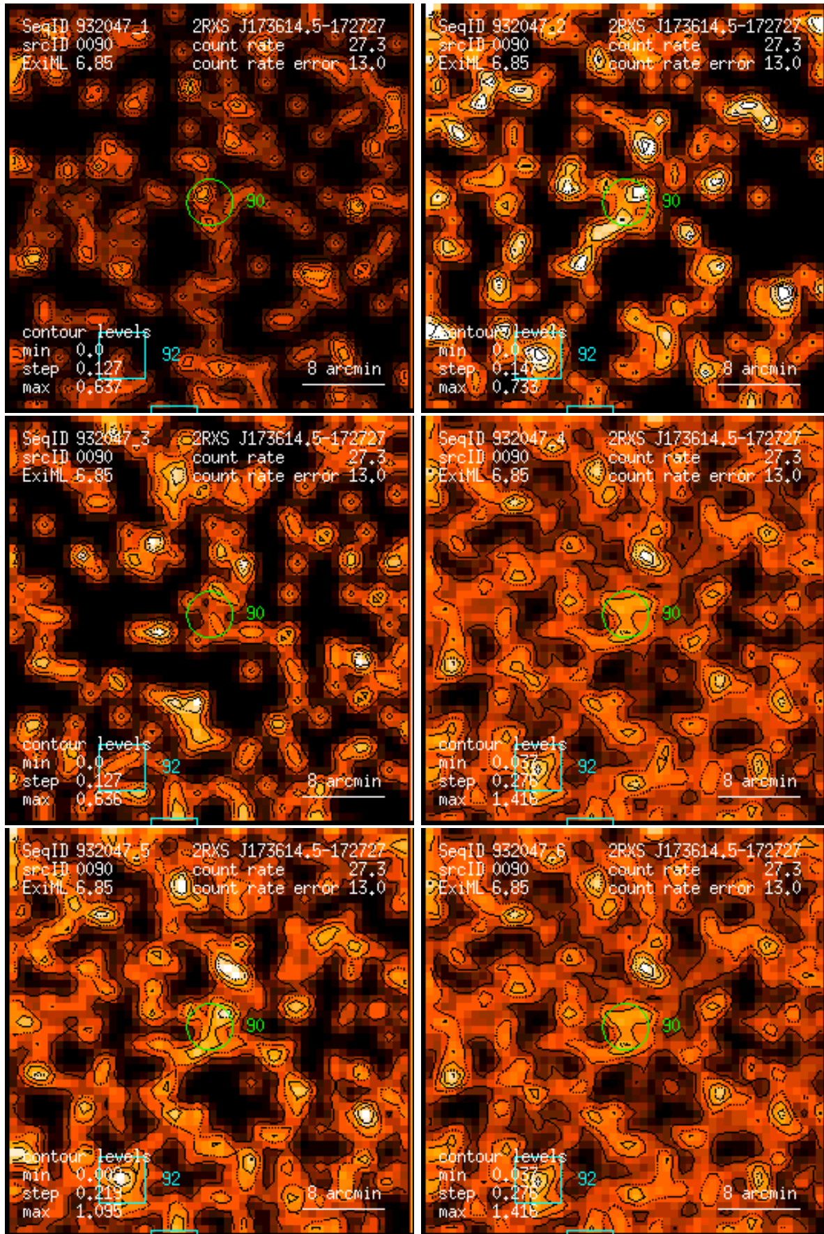
Figure 90: RASS 932047: detection 0090: band rate images, Gaussian filter: (1) PSPC channels 11 – 41, (2) 52 – 90, (3) 91 – 201, (4) 11 – 235, (5) 52 – 201, (6) 11 – 201. Broad band rates in counts/ks. Band rate contour levels in counts/ks/arcmin 2 .
