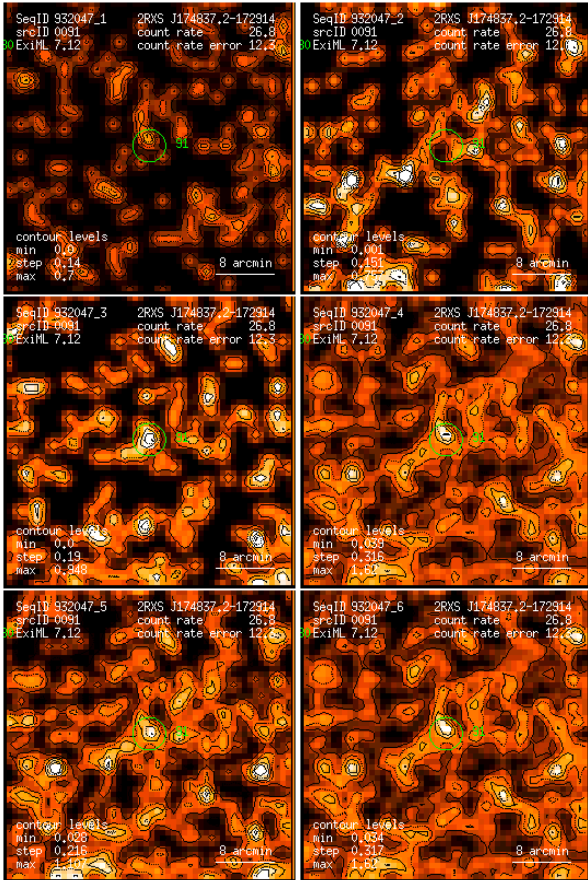
Figure 91: RASS 932047: detection 0091: band rate images, Gaussian filter: (1) PSPC channels 11 – 41, (2) 52 – 90, (3) 91 – 201, (4) 11 – 235, (5) 52 – 201, (6) 11 – 201. Broad band rates in counts/ks. Band rate contour levels in counts/ks/arcmin 2 .
