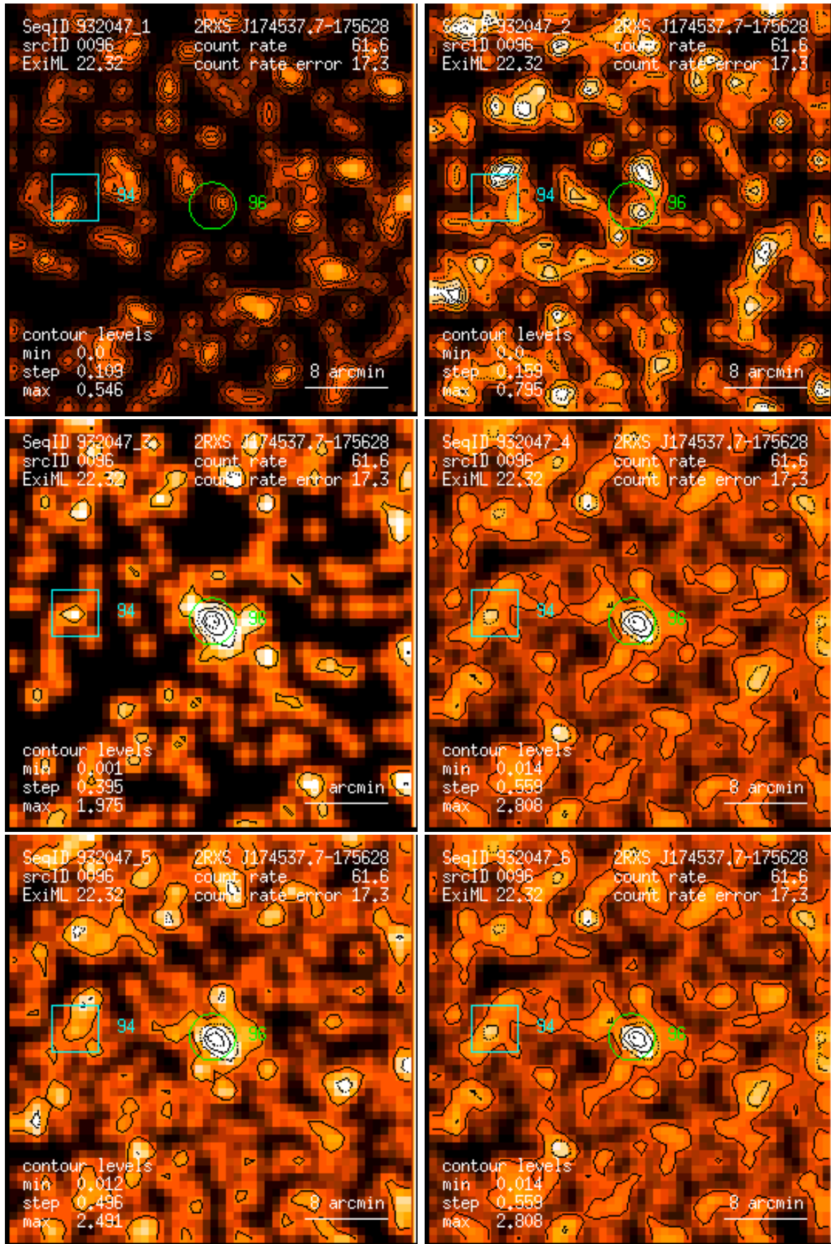
Figure 96: RASS 932047: detection 0096: band rate images, Gaussian filter: (1) PSPC channels 11 – 41, (2) 52 – 90, (3) 91 – 201, (4) 11 – 235, (5) 52 – 201, (6) 11 – 201. Broad band rates in counts/ks. Band rate contour levels in counts/ks/arcmin 2 .
