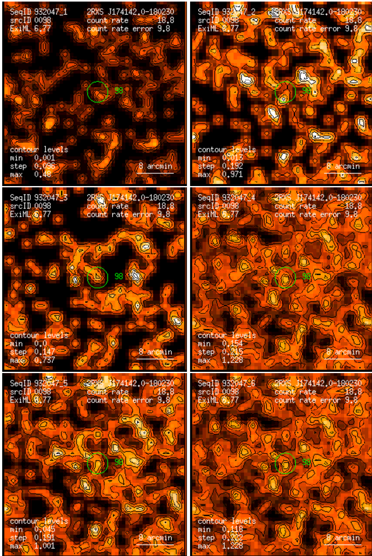
Figure 98: RASS 932047: detection 0098: band rate images, Gaussian filter: (1) PSPC channels 11 – 41, (2) 52 – 90, (3) 91 – 201, (4) 11 – 235, (5) 52 – 201, (6) 11 – 201. Broad band rates in counts/ks. Band rate contour levels in counts/ks/arcmin 2 .
