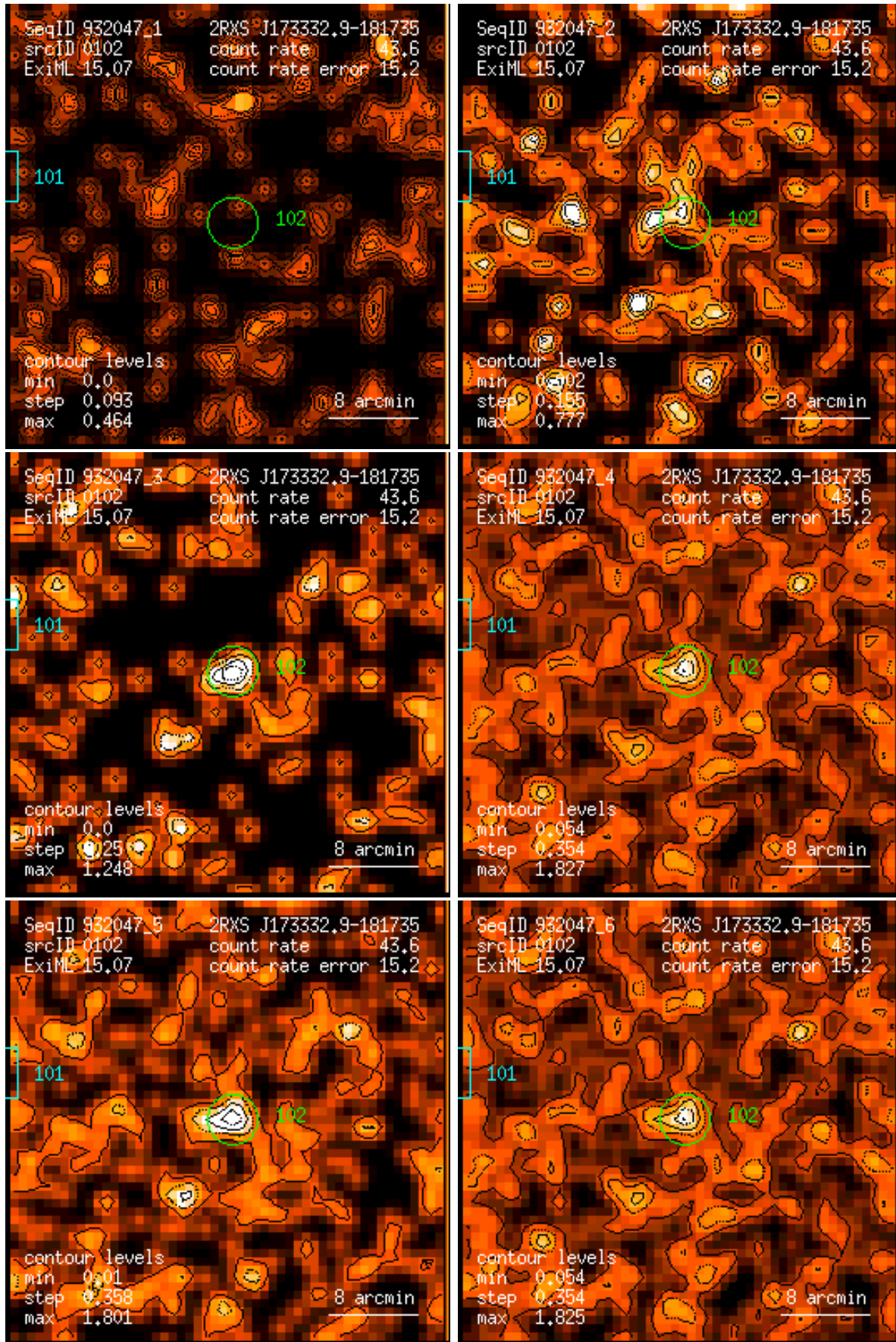
Figure 102: RASS 932047: detection 0102: band rate images, Gaussian filter: (1) PSPC channels 11 – 41, (2) 52 – 90, (3) 91 – 201, (4) 11 – 235, (5) 52 – 201, (6) 11 – 201. Broad band rates in counts/ks. Band rate contour levels in counts/ks/arcmin 2 .
