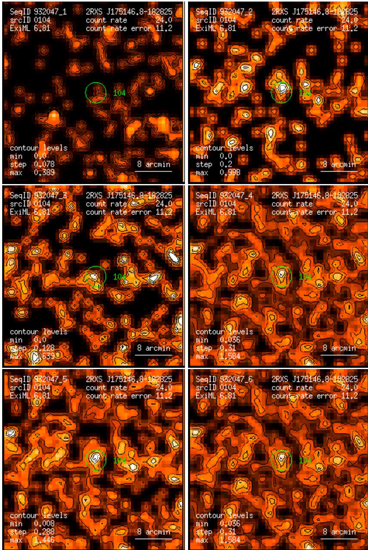
Figure 104: RASS 932047: detection 0104: band rate images, Gaussian filter: (1) PSPC channels 11 – 41, (2) 52 – 90, (3) 91 – 201, (4) 11 – 235, (5) 52 – 201, (6) 11 – 201. Broad band rates in counts/ks. Band rate contour levels in counts/ks/arcmin 2 .
