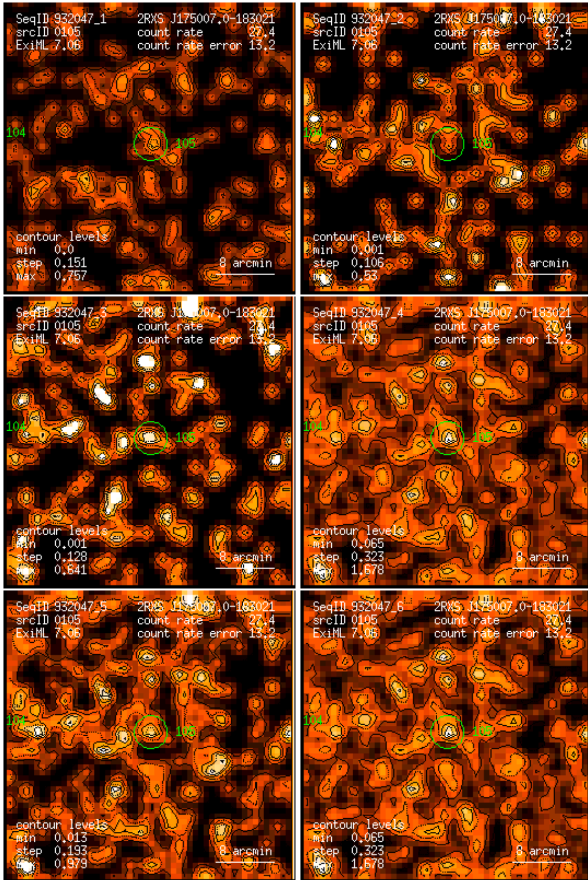
Figure 105: RASS 932047: detection 0105: band rate images, Gaussian filter: (1) PSPC channels 11 – 41, (2) 52 – 90, (3) 91 – 201, (4) 11 – 235, (5) 52 – 201, (6) 11 – 201. Broad band rates in counts/ks. Band rate contour levels in counts/ks/arcmin 2 .
