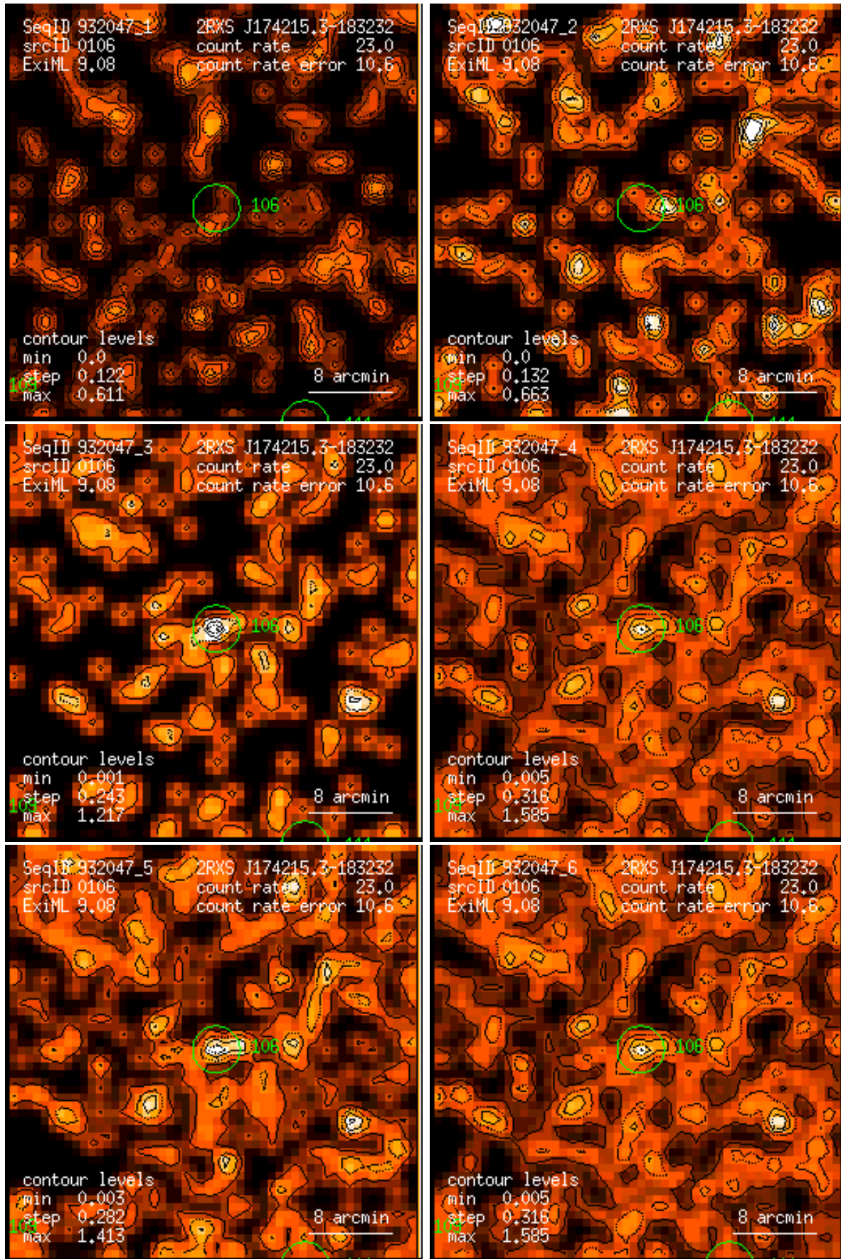
Figure 106: RASS 932047: detection 0106: band rate images, Gaussian filter: (1) PSPC channels 11 – 41, (2) 52 – 90, (3) 91 – 201, (4) 11 – 235, (5) 52 – 201, (6) 11 – 201. Broad band rates in counts/ks. Band rate contour levels in counts/ks/arcmin 2 .
