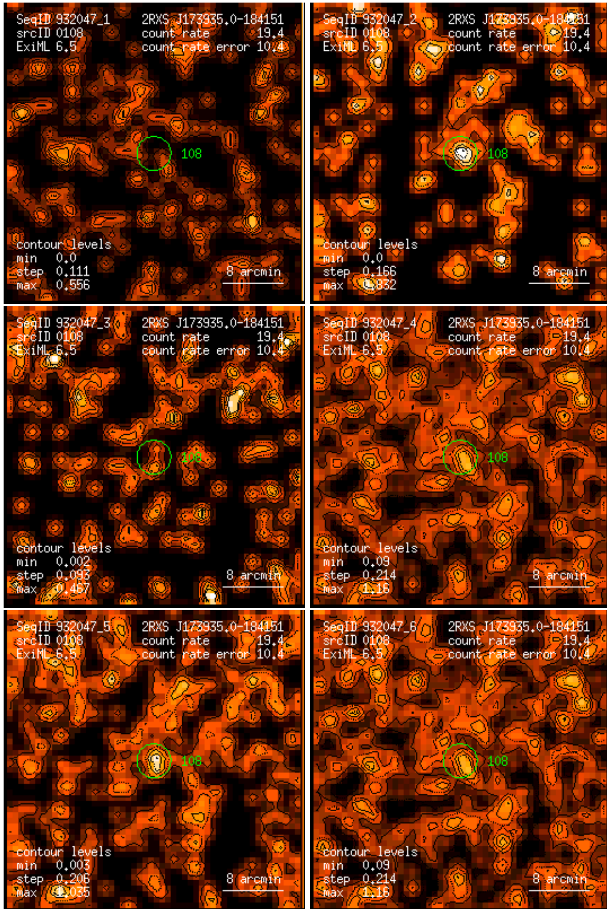
Figure 108: RASS 932047: detection 0108: band rate images, Gaussian filter: (1) PSPC channels 11 – 41, (2) 52 – 90, (3) 91 – 201, (4) 11 – 235, (5) 52 – 201, (6) 11 – 201. Broad band rates in counts/ks. Band rate contour levels in counts/ks/arcmin 2 .
