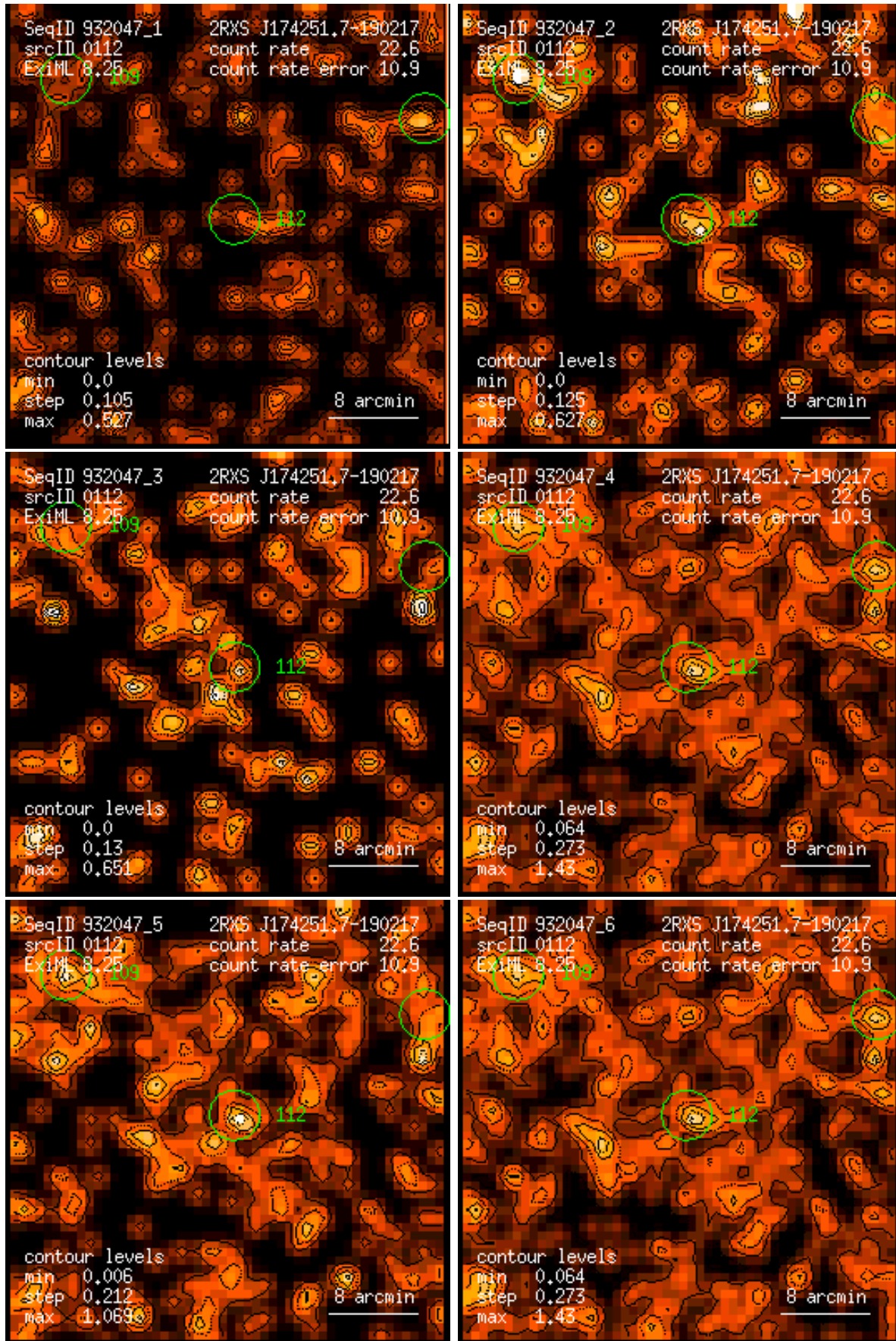
Figure 112: RASS 932047: detection 0112: band rate images, Gaussian filter: (1) PSPC channels 11 – 41, (2) 52 – 90, (3) 91 – 201, (4) 11 – 235, (5) 52 – 201, (6) 11 – 201. Broad band rates in counts/ks. Band rate contour levels in counts/ks/arcmin 2 .
