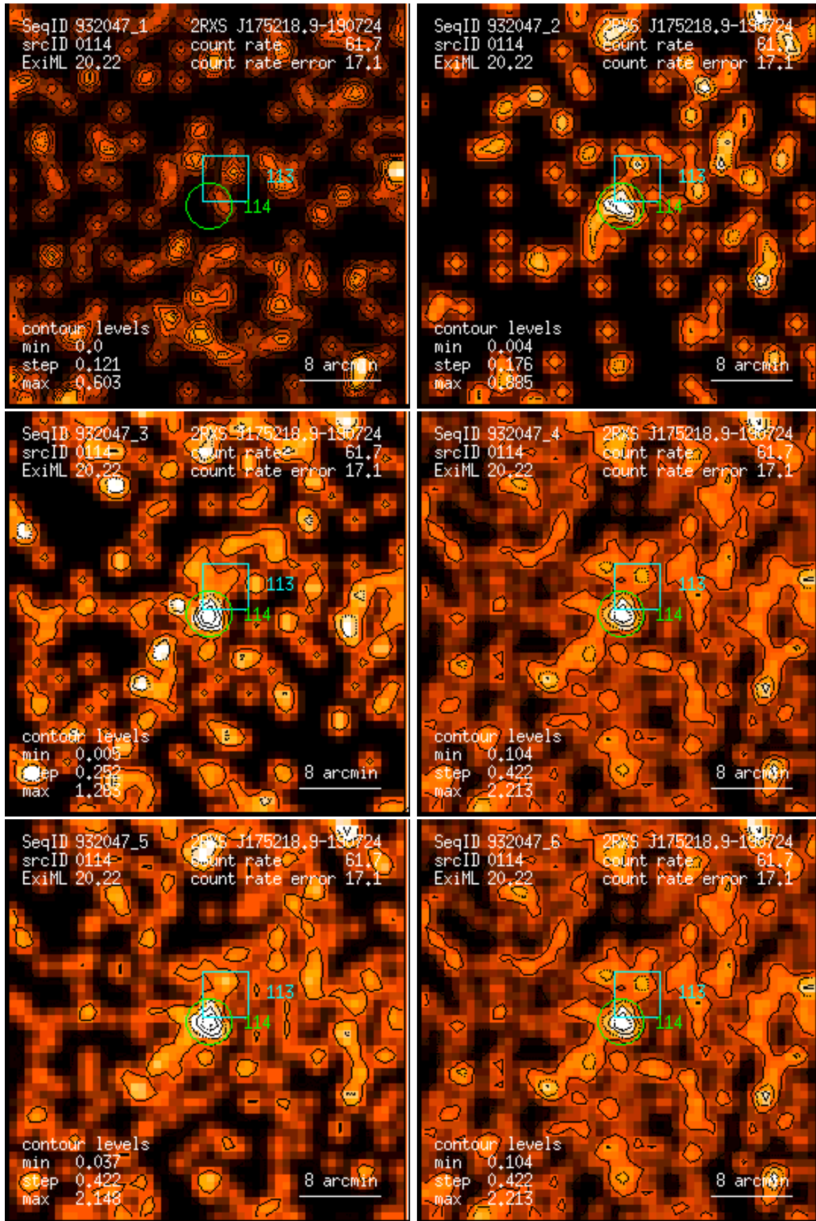
Figure 114: RASS 932047: detection 0114: band rate images, Gaussian filter: (1) PSPC channels 11 – 41, (2) 52 – 90, (3) 91 – 201, (4) 11 – 235, (5) 52 – 201, (6) 11 – 201. Broad band rates in counts/ks. Band rate contour levels in counts/ks/arcmin 2 .
