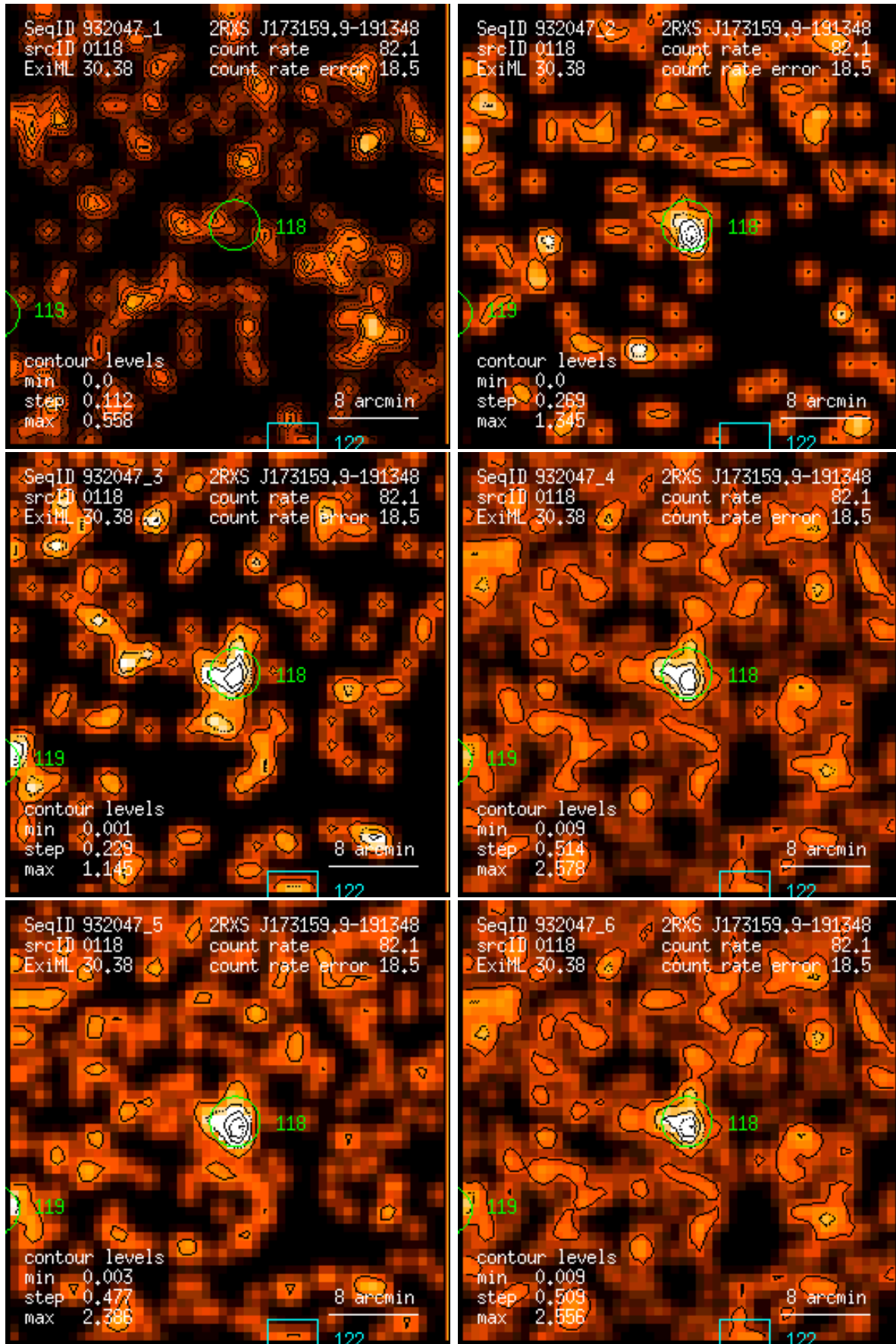
Figure 118: RASS 932047: detection 0118: band rate images, Gaussian filter: (1) PSPC channels 11 – 41, (2) 52 – 90, (3) 91 – 201, (4) 11 – 235, (5) 52 – 201, (6) 11 – 201. Broad band rates in counts/ks. Band rate contour levels in counts/ks/arcmin 2 .
