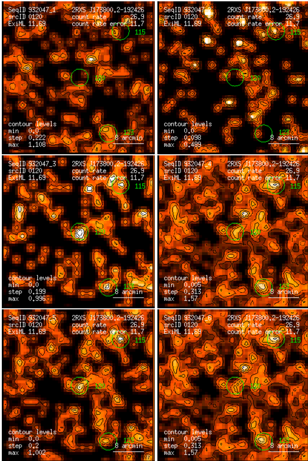
Figure 120: RASS 932047: detection 0120: band rate images, Gaussian filter: (1) PSPC channels 11 – 41, (2) 52 – 90, (3) 91 – 201, (4) 11 – 235, (5) 52 – 201, (6) 11 – 201. Broad band rates in counts/ks. Band rate contour levels in counts/ks/arcmin 2 .
