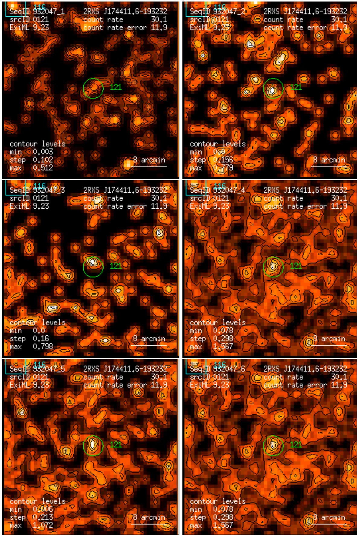
Figure 121: RASS 932047: detection 0121: band rate images, Gaussian filter: (1) PSPC channels 11 – 41, (2) 52 – 90, (3) 91 – 201, (4) 11 – 235, (5) 52 – 201, (6) 11 – 201. Broad band rates in counts/ks. Band rate contour levels in counts/ks/arcmin 2 .
