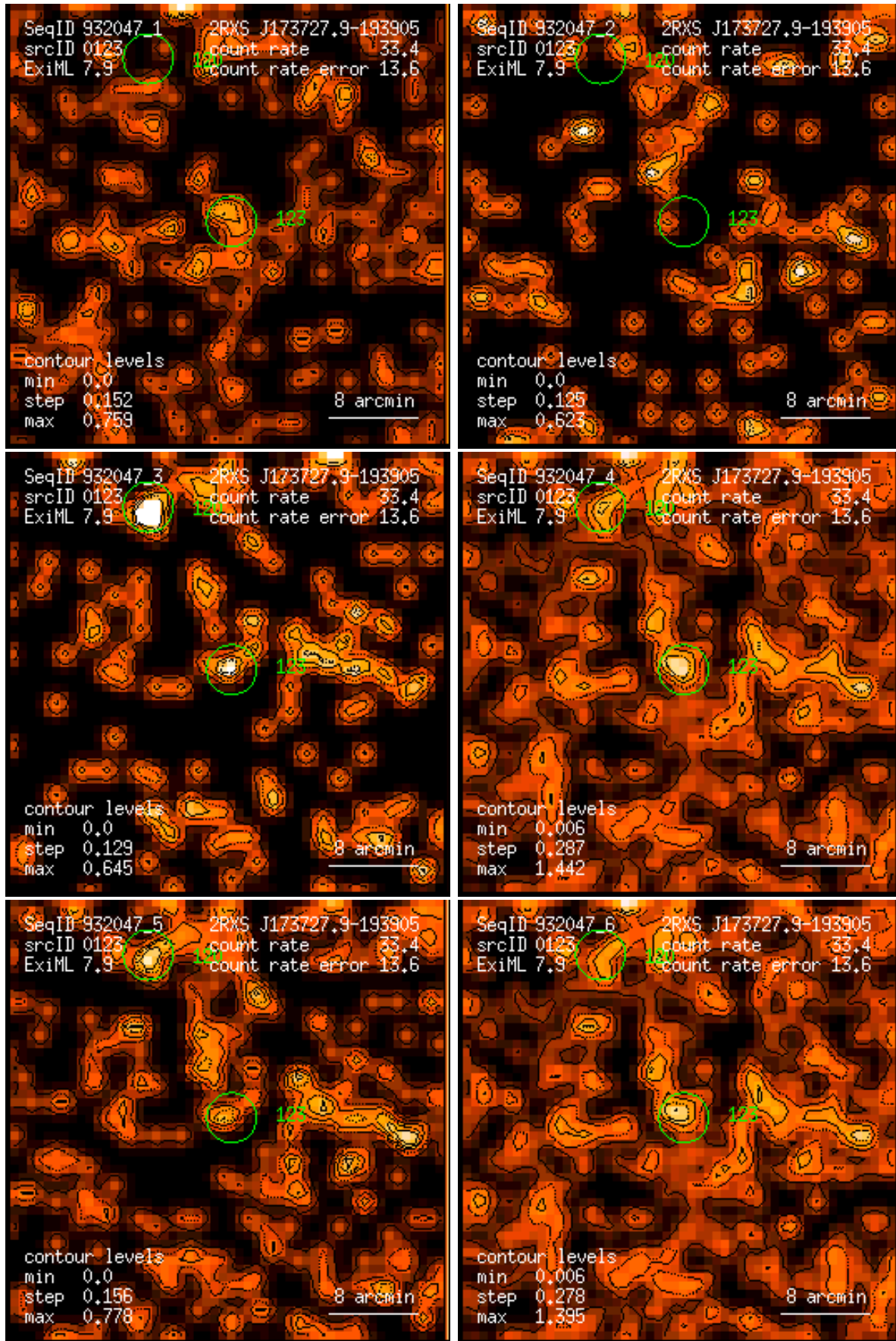
Figure 123: RASS 932047: detection 0123: band rate images, Gaussian filter: (1) PSPC channels 11 – 41, (2) 52 – 90, (3) 91 – 201, (4) 11 – 235, (5) 52 – 201, (6) 11 – 201. Broad band rates in counts/ks. Band rate contour levels in counts/ks/arcmin 2 .
