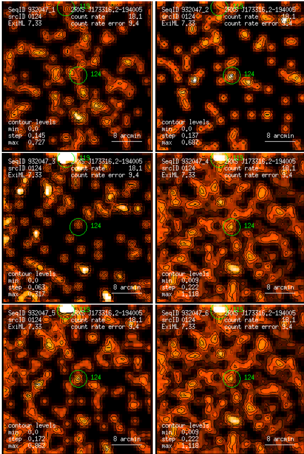
Figure 124: RASS 932047: detection 0124: band rate images, Gaussian filter: (1) PSPC channels 11 – 41, (2) 52 – 90, (3) 91 – 201, (4) 11 – 235, (5) 52 – 201, (6) 11 – 201. Broad band rates in counts/ks. Band rate contour levels in counts/ks/arcmin 2 .
