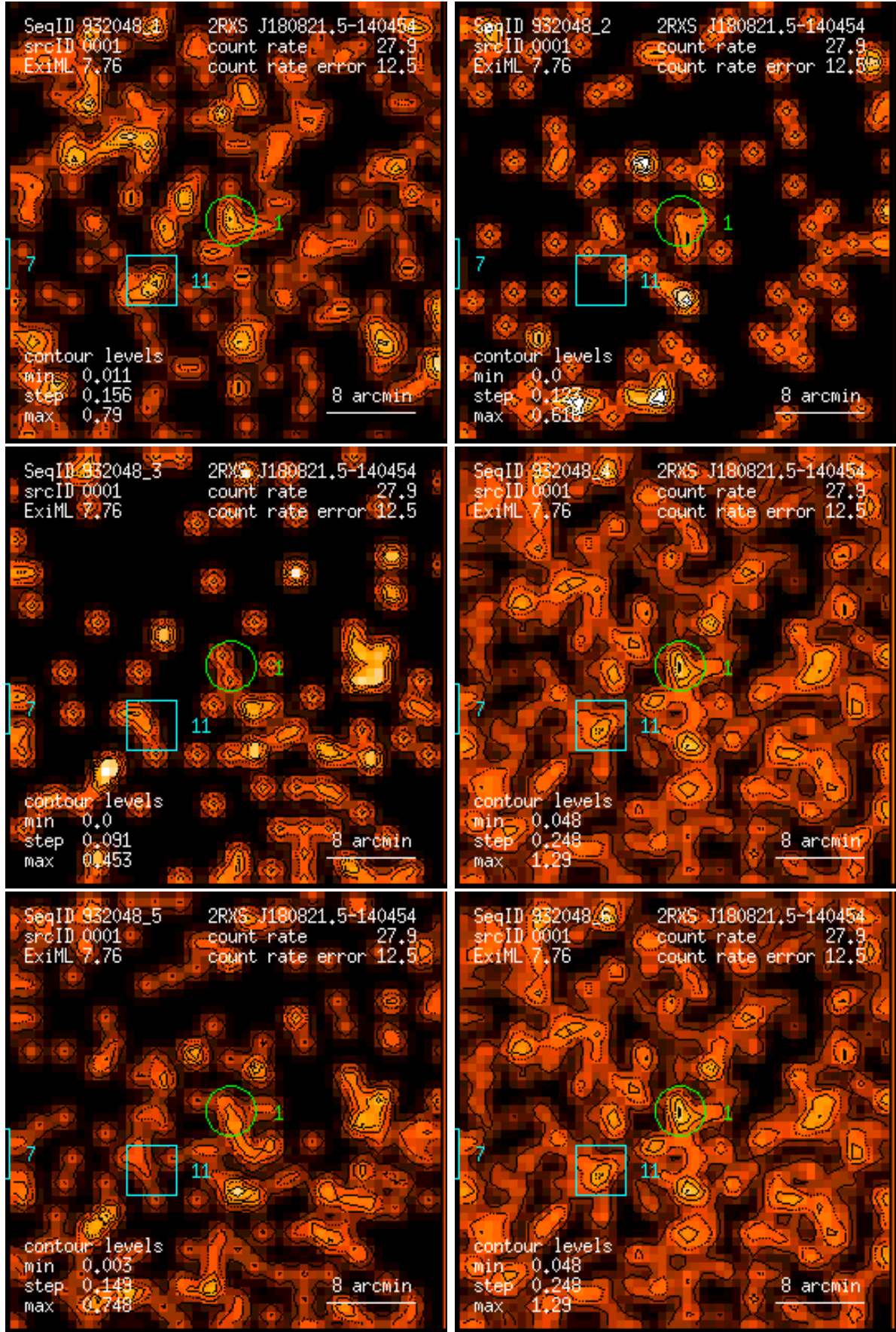
Figure 1: RASS 932048: detection 0001: band rate images, Gaussian filter: (1) PSPC channels 11 – 41, (2) 52 – 90, (3) 91 – 201, (4) 11 – 235, (5) 52 – 201, (6) 11 – 201. Broad band rates in counts/ks. Band rate contour levels in counts/ks/arcmin 2 .
