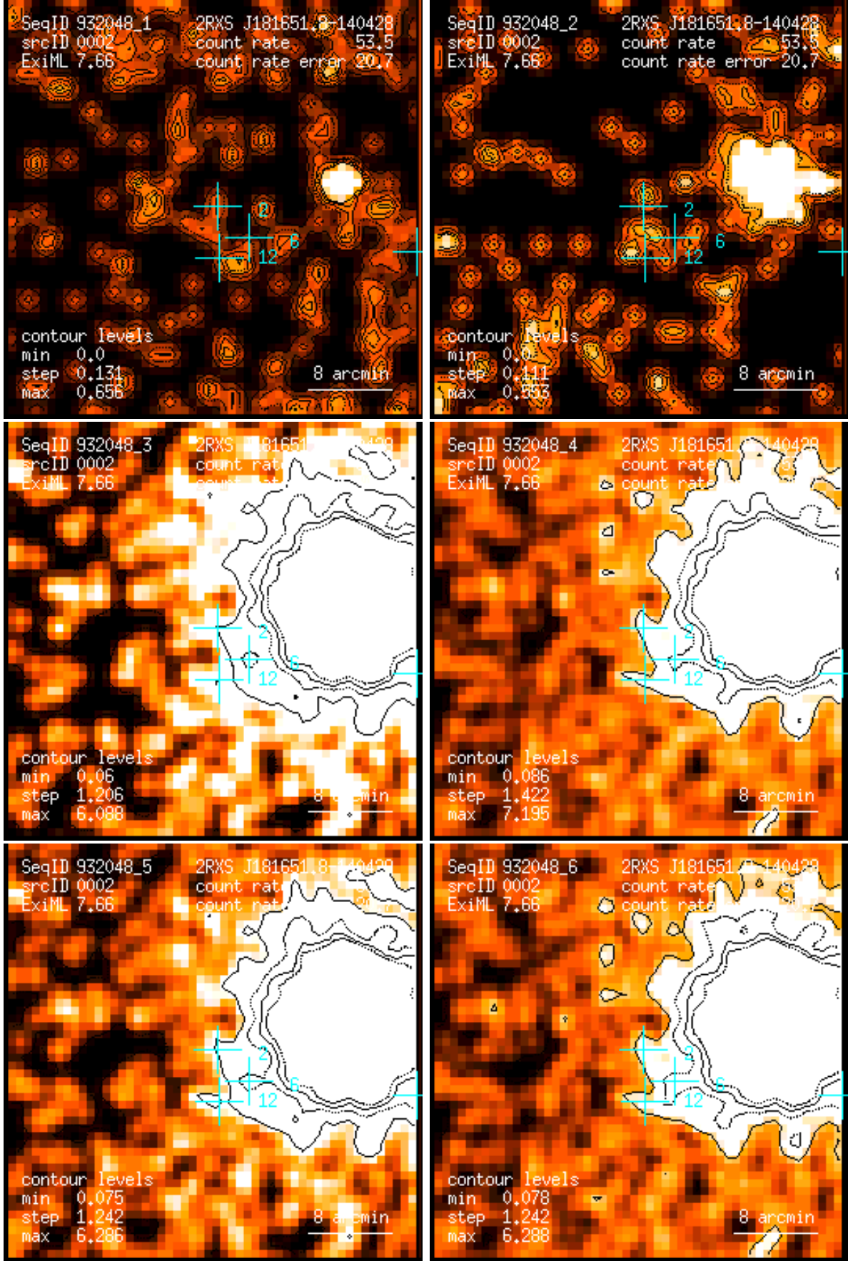
Figure 2: RASS 932048: detection 0002: band rate images, Gaussian filter: (1) PSPC channels 11 – 41, (2) 52 – 90, (3) 91 – 201, (4) 11 – 235, (5) 52 – 201, (6) 11 – 201. Broad band rates in counts/ks. Band rate contour levels in counts/ks/arcmin 2 .
