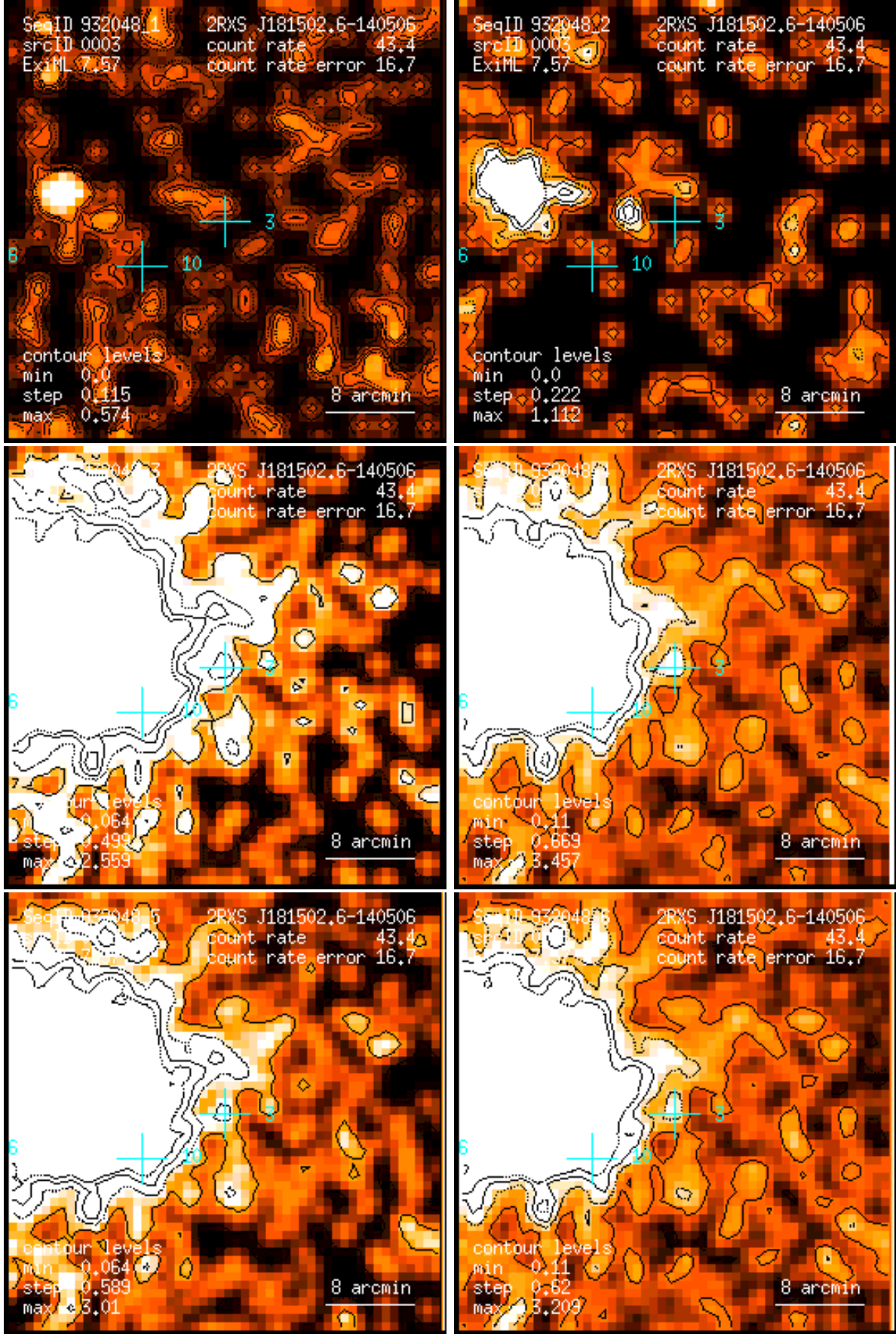
Figure 3: RASS 932048: detection 0003: band rate images, Gaussian filter: (1) PSPC channels 11 – 41, (2) 52 – 90, (3) 91 – 201, (4) 11 – 235, (5) 52 – 201, (6) 11 – 201. Broad band rates in counts/ks. Band rate contour levels in counts/ks/arcmin 2 .
