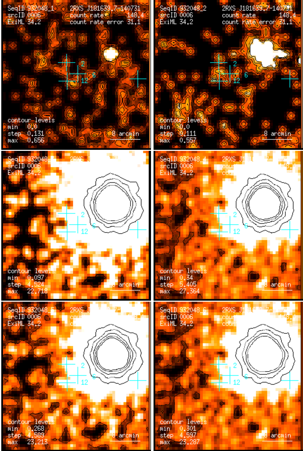
Figure 6: RASS 932048: detection 0006: band rate images, Gaussian filter: (1) PSPC channels 11 – 41, (2) 52 – 90, (3) 91 – 201, (4) 11 – 235, (5) 52 – 201, (6) 11 – 201. Broad band rates in counts/ks. Band rate contour levels in counts/ks/arcmin 2 .
