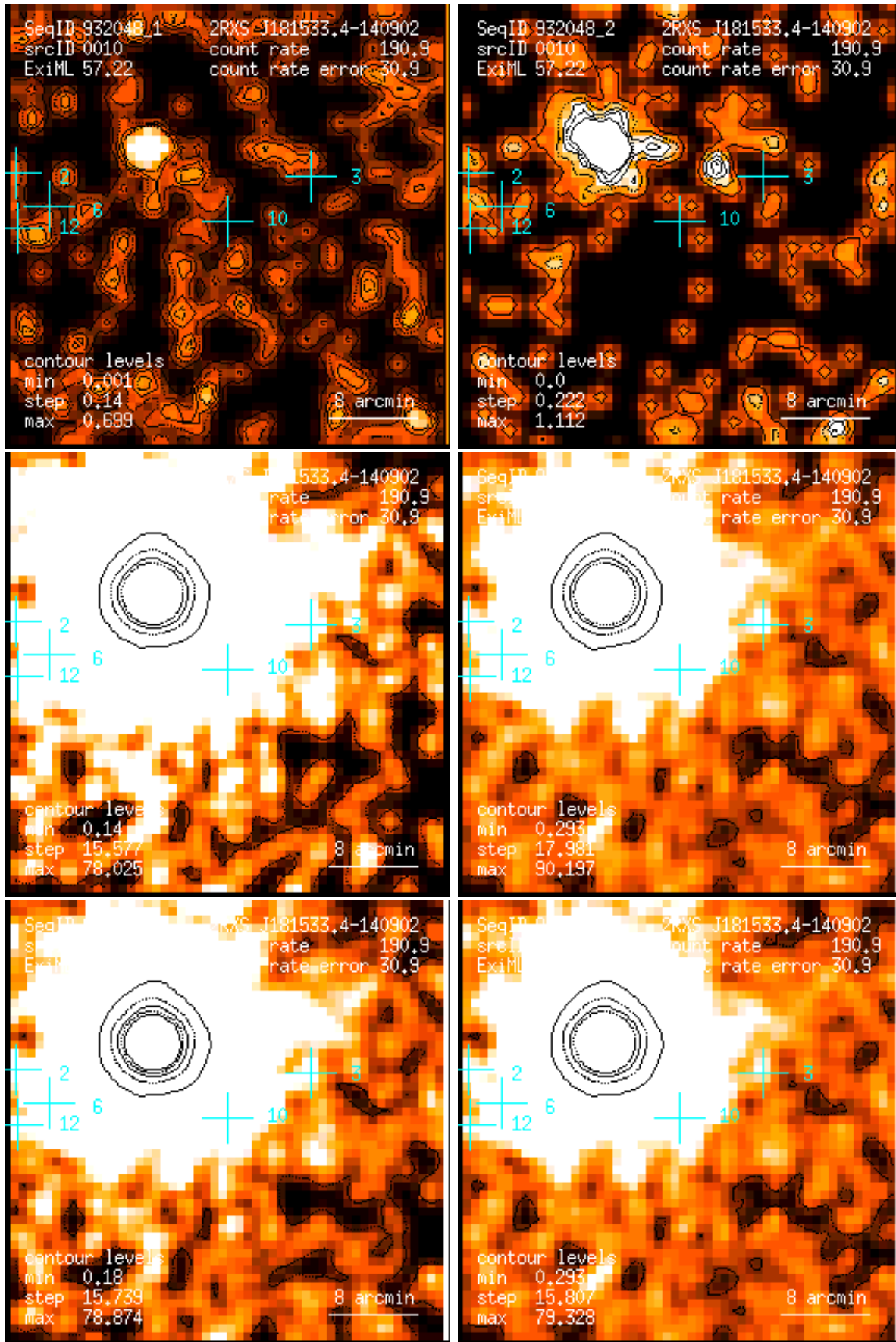
Figure 10: RASS 932048: detection 0010: band rate images, Gaussian filter: (1) PSPC channels 11 – 41, (2) 52 – 90, (3) 91 – 201, (4) 11 – 235, (5) 52 – 201, (6) 11 – 201. Broad band rates in counts/ks. Band rate contour levels in counts/ks/arcmin 2 .
