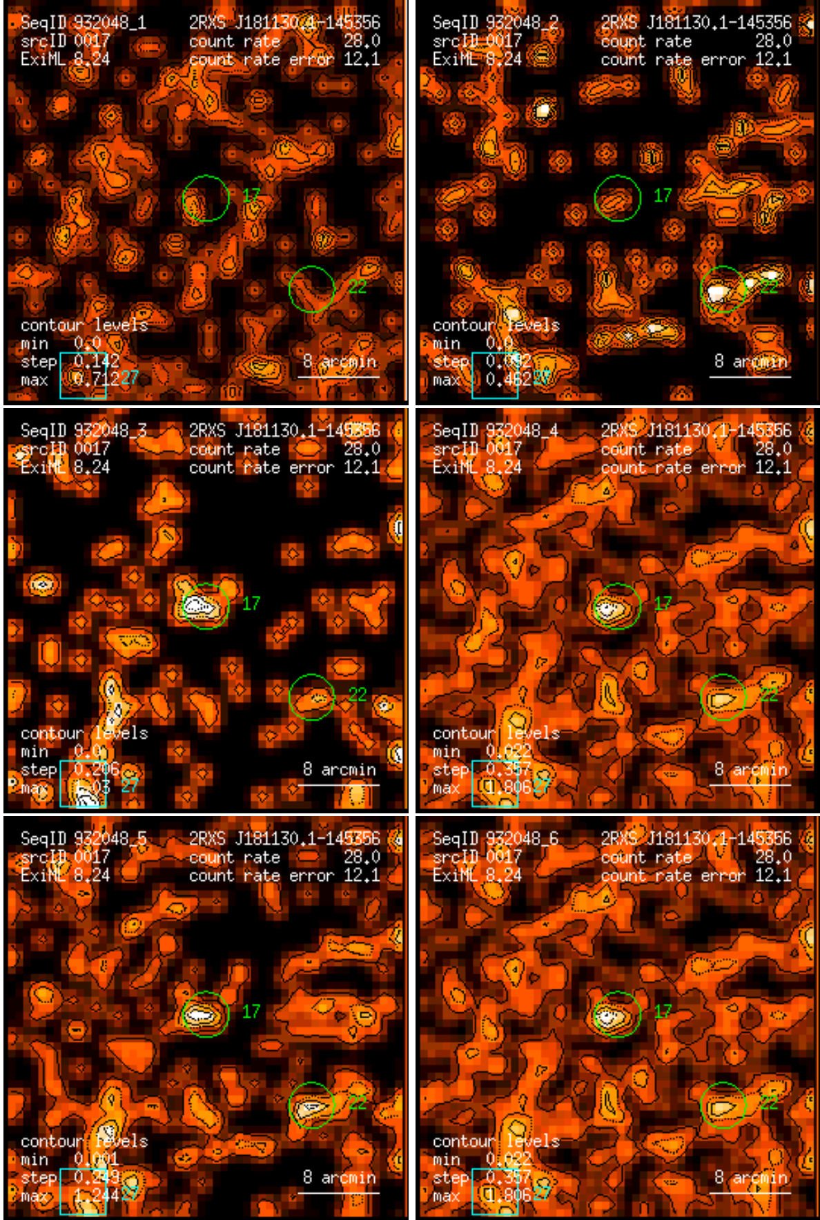
Figure 17: RASS 932048: detection 0017: band rate images, Gaussian filter: (1) PSPC channels 11 – 41, (2) 52 – 90, (3) 91 – 201, (4) 11 – 235, (5) 52 – 201, (6) 11 – 201. Broad band rates in counts/ks. Band rate contour levels in counts/ks/arcmin 2 .
