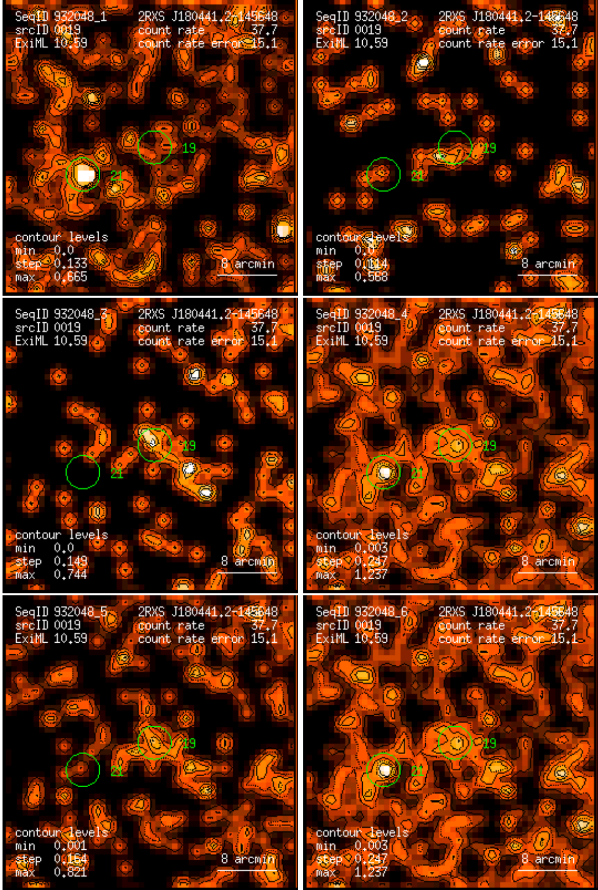
Figure 19: RASS 932048: detection 0019: band rate images, Gaussian filter: (1) PSPC channels 11 – 41, (2) 52 – 90, (3) 91 – 201, (4) 11 – 235, (5) 52 – 201, (6) 11 – 201. Broad band rates in counts/ks. Band rate contour levels in counts/ks/arcmin 2 .
