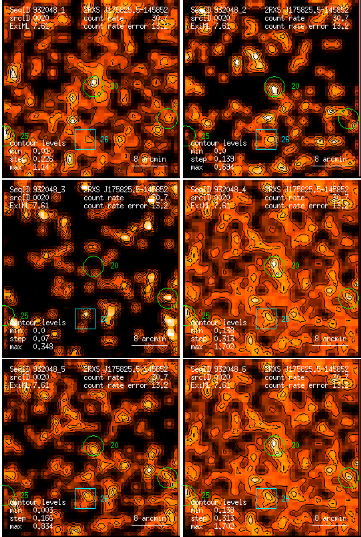
Figure 20: RASS 932048: detection 0020: band rate images, Gaussian filter: (1) PSPC channels 11 – 41, (2) 52 – 90, (3) 91 – 201, (4) 11 – 235, (5) 52 – 201, (6) 11 – 201. Broad band rates in counts/ks. Band rate contour levels in counts/ks/arcmin 2 .
