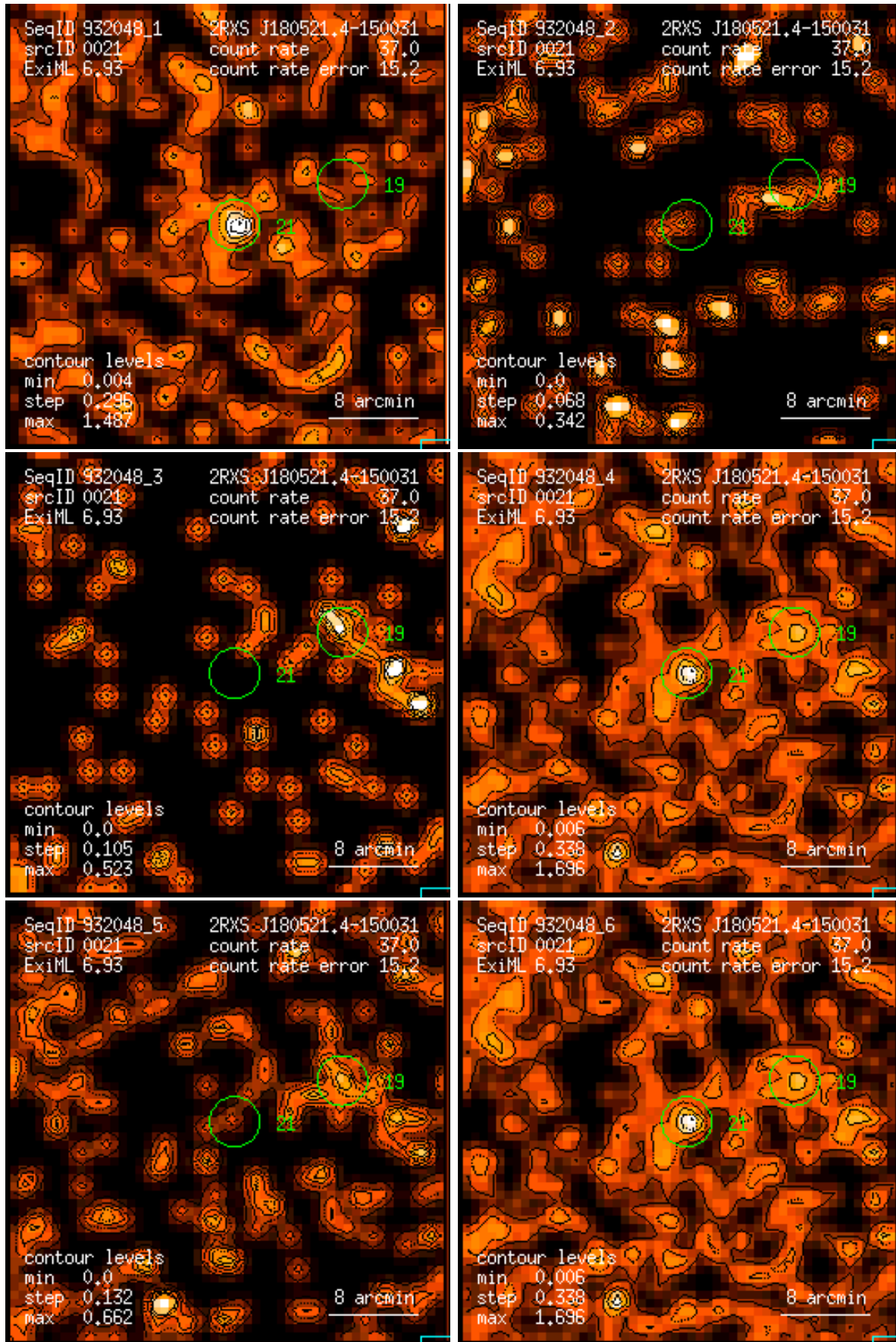
Figure 21: RASS 932048: detection 0021: band rate images, Gaussian filter: (1) PSPC channels 11 – 41, (2) 52 – 90, (3) 91 – 201, (4) 11 – 235, (5) 52 – 201, (6) 11 – 201. Broad band rates in counts/ks. Band rate contour levels in counts/ks/arcmin 2 .
