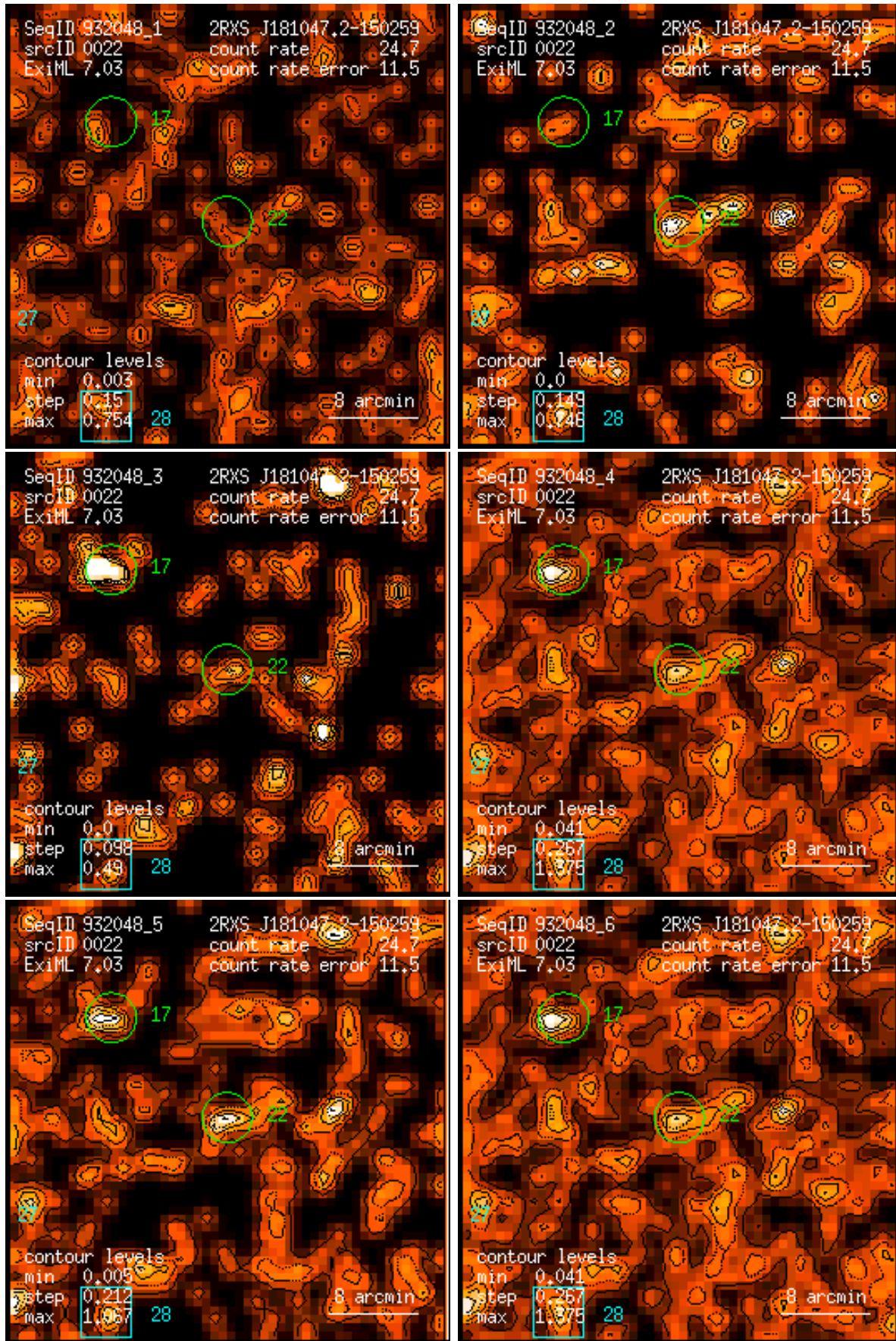
Figure 22: RASS 932048: detection 0022: band rate images, Gaussian filter: (1) PSPC channels 11 – 41, (2) 52 – 90, (3) 91 – 201, (4) 11 – 235, (5) 52 – 201, (6) 11 – 201. Broad band rates in counts/ks. Band rate contour levels in counts/ks/arcmin 2 .
