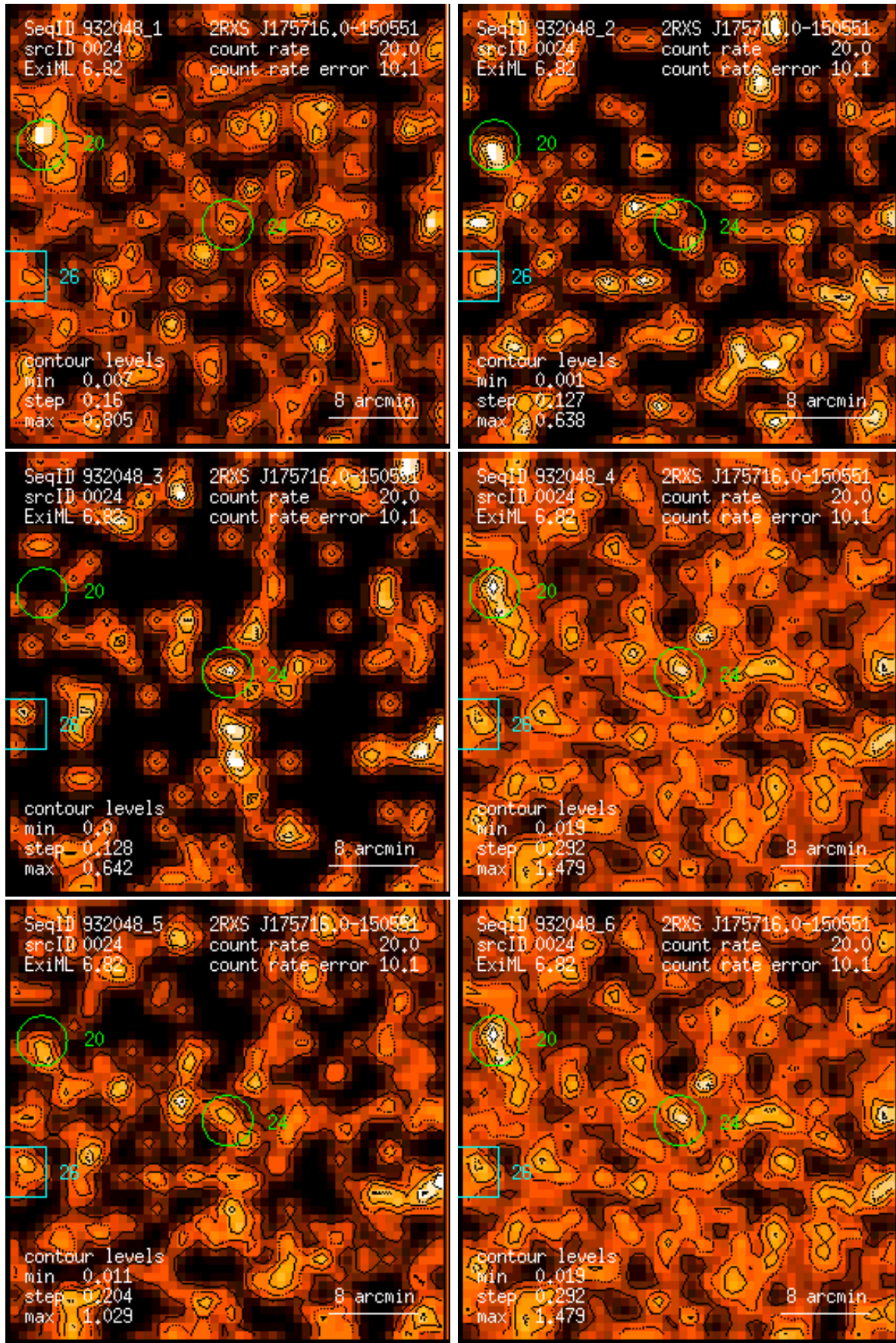
Figure 24: RASS 932048: detection 0024: band rate images, Gaussian filter: (1) PSPC channels 11 – 41, (2) 52 – 90, (3) 91 – 201, (4) 11 – 235, (5) 52 – 201, (6) 11 – 201. Broad band rates in counts/ks. Band rate contour levels in counts/ks/arcmin 2 .
