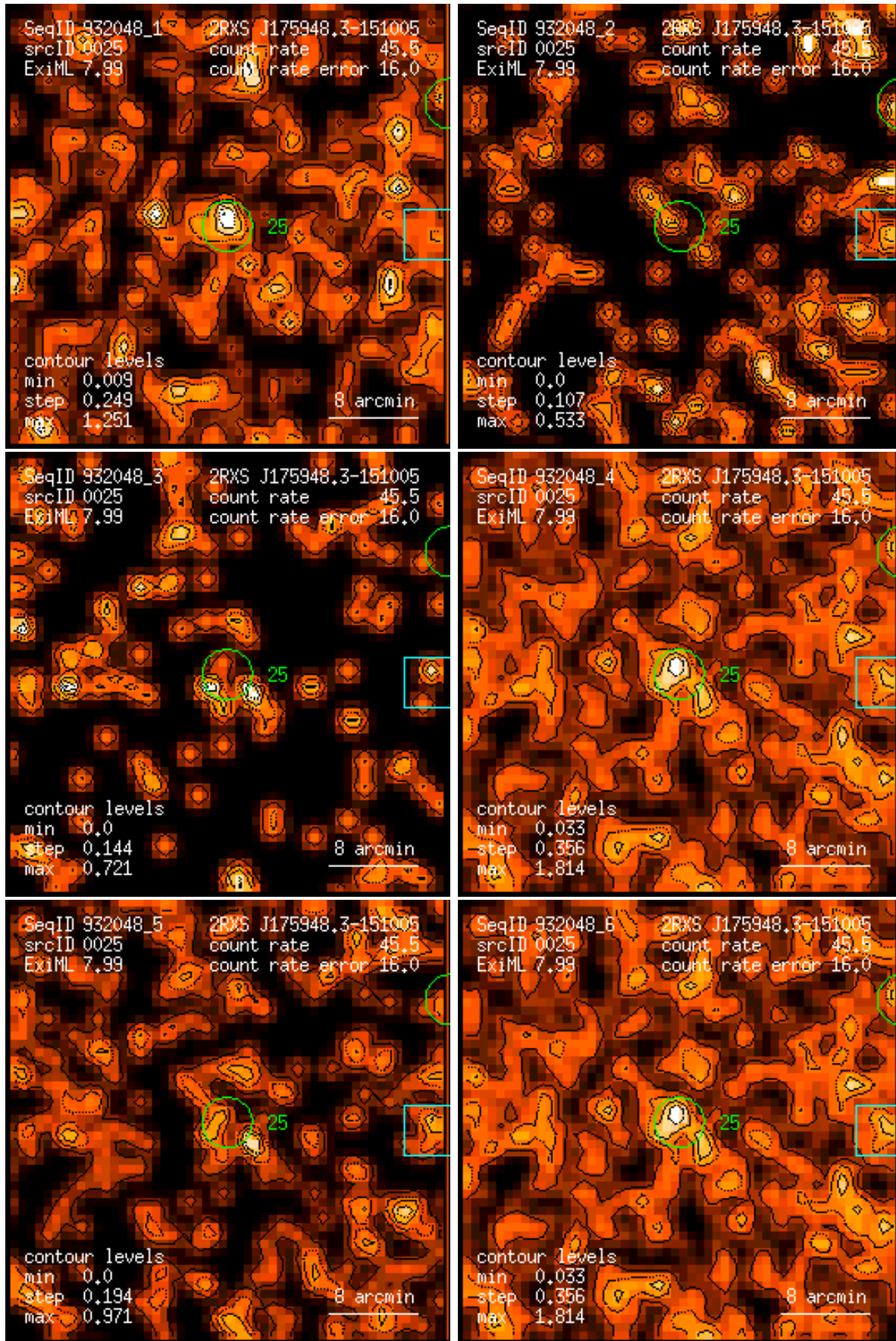
Figure 25: RASS 932048: detection 0025: band rate images, Gaussian filter: (1) PSPC channels 11 – 41, (2) 52 – 90, (3) 91 – 201, (4) 11 – 235, (5) 52 – 201, (6) 11 – 201. Broad band rates in counts/ks. Band rate contour levels in counts/ks/arcmin 2 .
