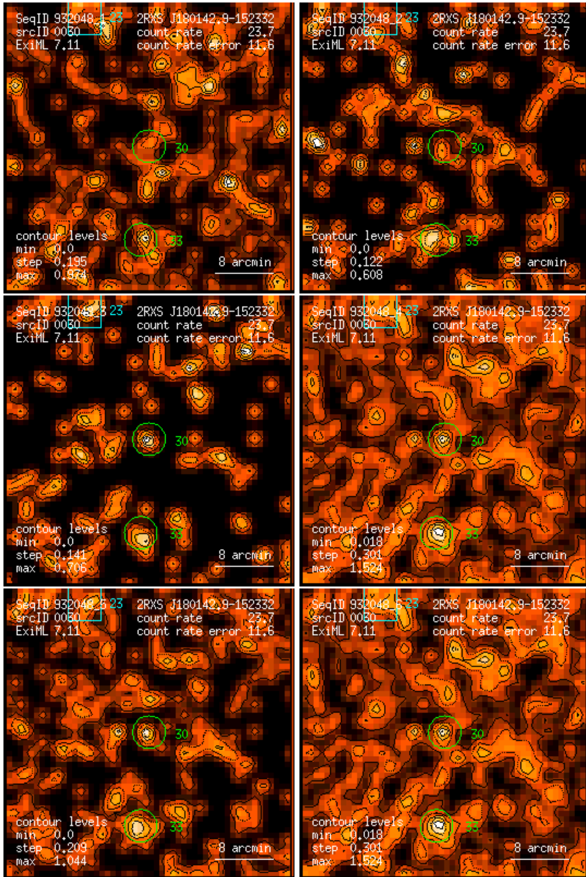
Figure 30: RASS 932048: detection 0030: band rate images, Gaussian filter: (1) PSPC channels 11 – 41, (2) 52 – 90, (3) 91 – 201, (4) 11 – 235, (5) 52 – 201, (6) 11 – 201. Broad band rates in counts/ks. Band rate contour levels in counts/ks/arcmin 2 .
