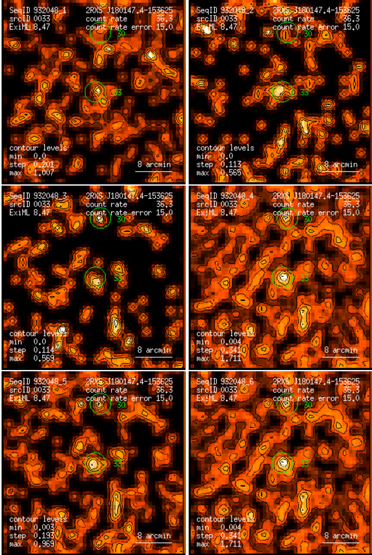
Figure 33: RASS 932048: detection 0033: band rate images, Gaussian filter: (1) PSPC channels 11 – 41, (2) 52 – 90, (3) 91 – 201, (4) 11 – 235, (5) 52 – 201, (6) 11 – 201. Broad band rates in counts/ks. Band rate contour levels in counts/ks/arcmin 2 .
