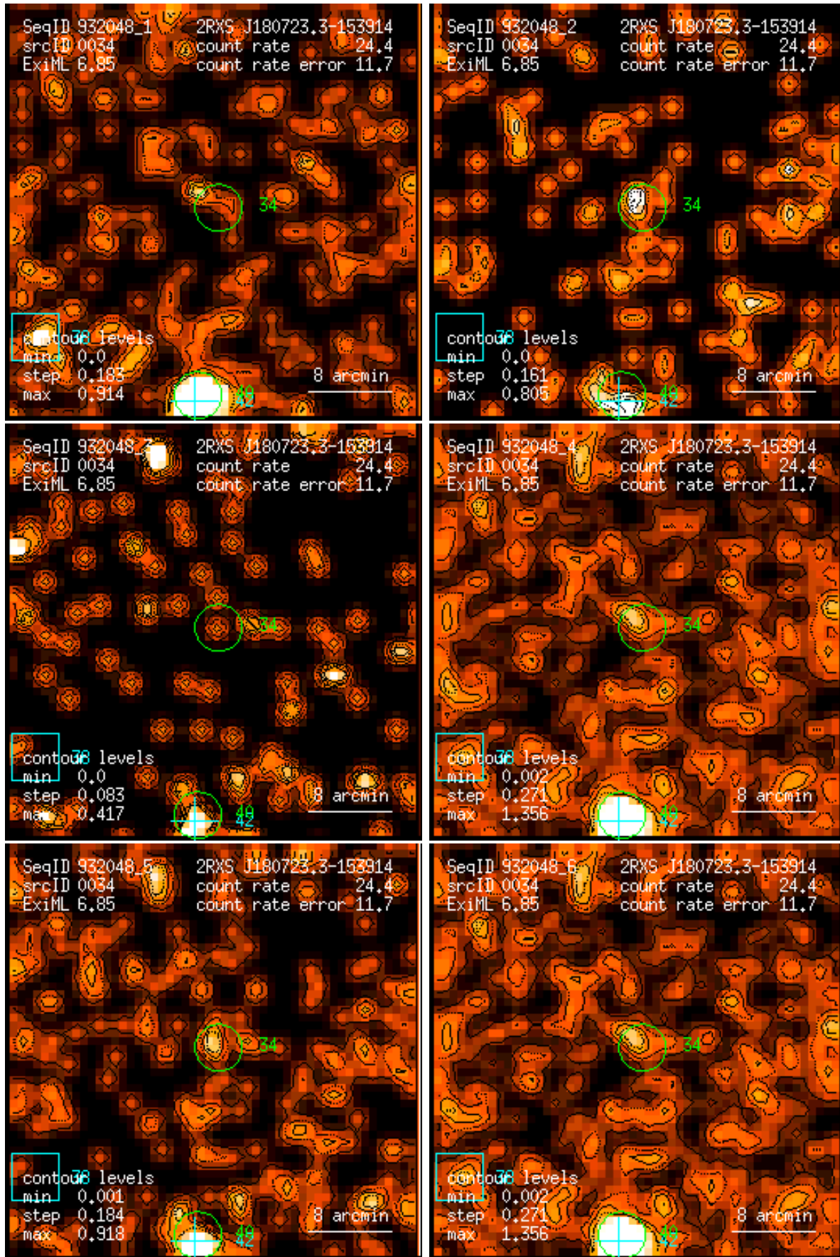
Figure 34: RASS 932048: detection 0034: band rate images, Gaussian filter: (1) PSPC channels 11 – 41, (2) 52 – 90, (3) 91 – 201, (4) 11 – 235, (5) 52 – 201, (6) 11 – 201. Broad band rates in counts/ks. Band rate contour levels in counts/ks/arcmin 2 .
