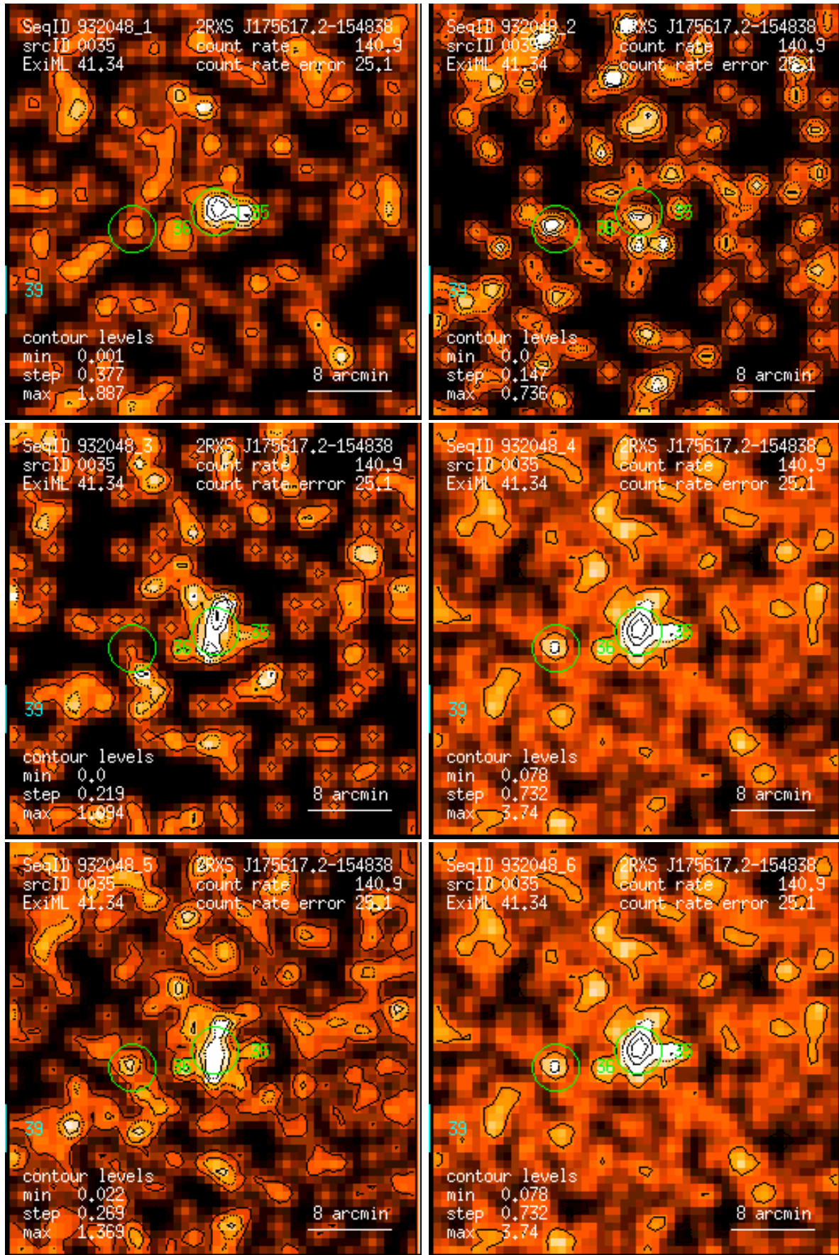
Figure 35: RASS 932048: detection 0035: band rate images, Gaussian filter: (1) PSPC channels 11 – 41, (2) 52 – 90, (3) 91 – 201, (4) 11 – 235, (5) 52 – 201, (6) 11 – 201. Broad band rates in counts/ks. Band rate contour levels in counts/ks/arcmin 2 .
