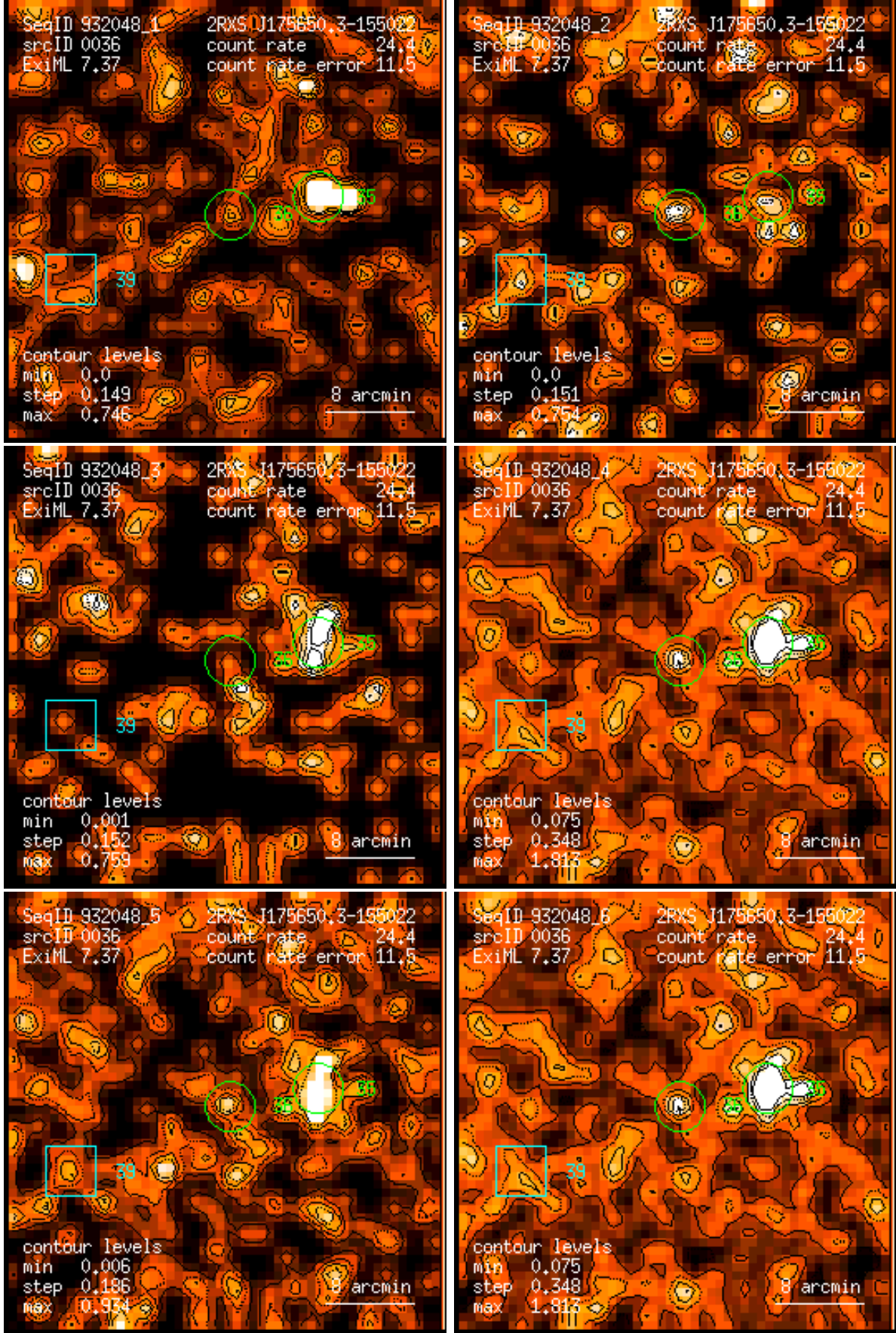
Figure 36: RASS 932048: detection 0036: band rate images, Gaussian filter: (1) PSPC channels 11 – 41, (2) 52 – 90, (3) 91 – 201, (4) 11 – 235, (5) 52 – 201, (6) 11 – 201. Broad band rates in counts/ks. Band rate contour levels in counts/ks/arcmin 2 .
